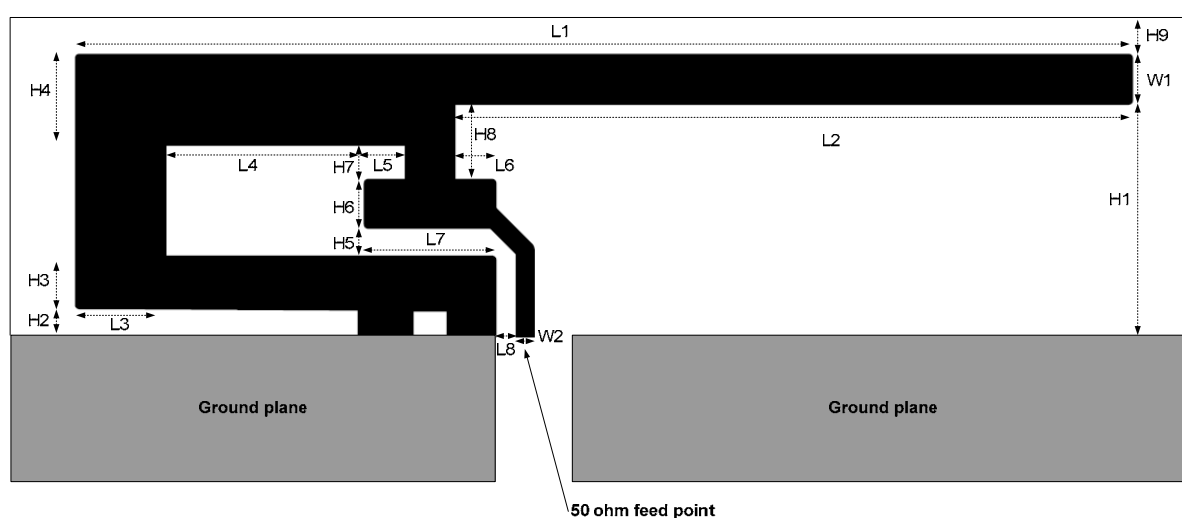
Figure 1. IFA Dimensions
