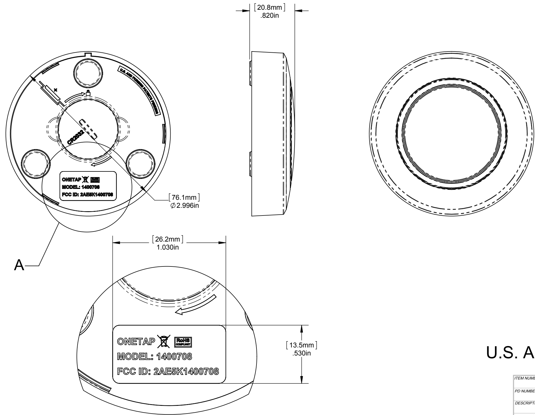
DETAIL A SCALE 2 : 1
