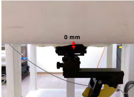
Fig.6 EUT Front side_3 to flat phantom
