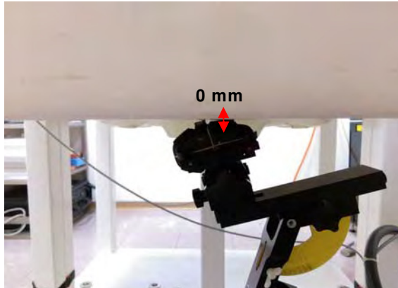
Fig.9 EUT Bottom side_3 to flat phantom
