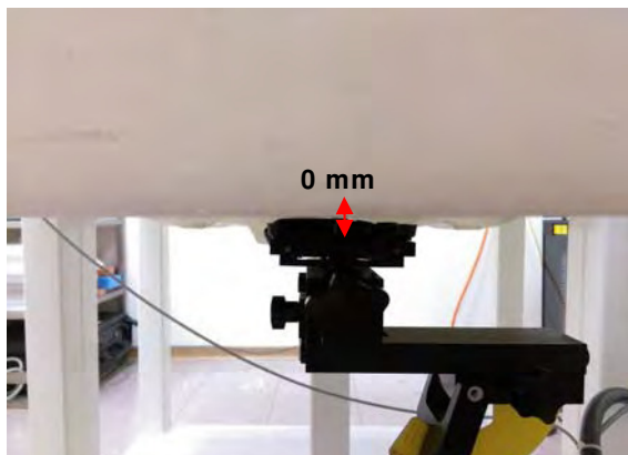
Fig.3 EUT Front side_1 to flat phantom
