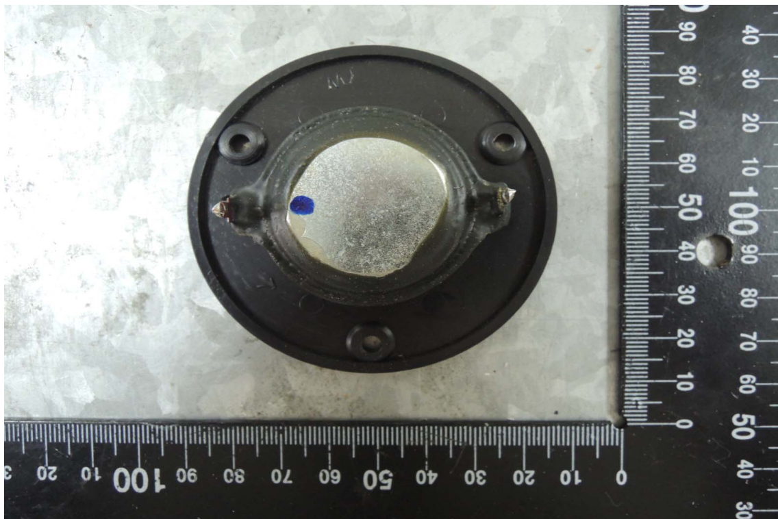
Open View of EUT – 7
