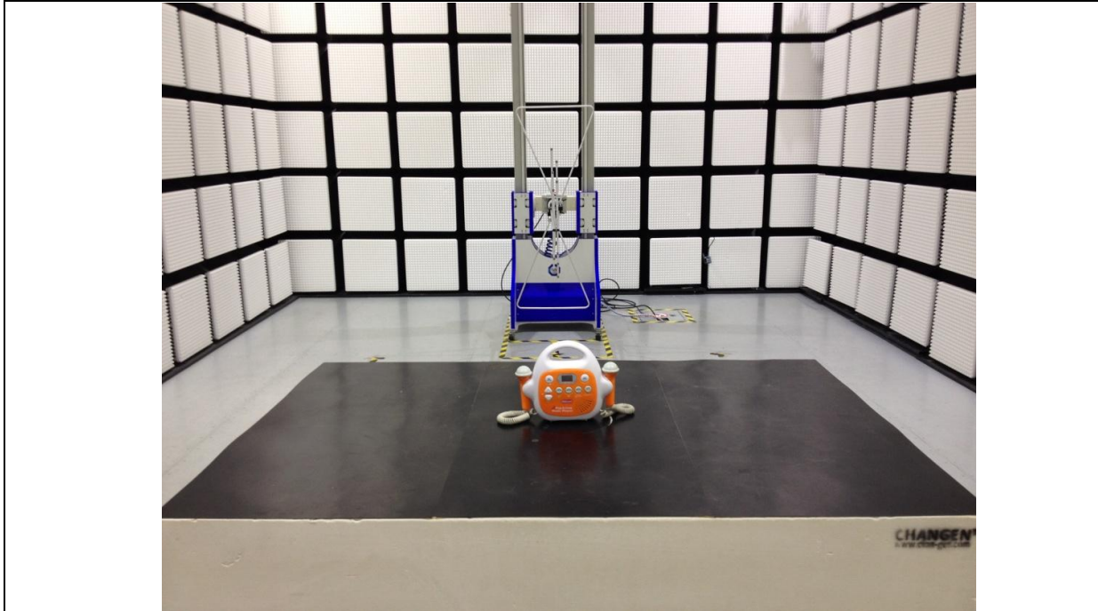
Radiated Emission Test (above 1G)
