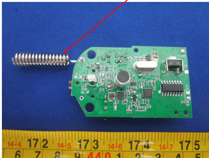
EUT- Main Board Top And Antenna View
