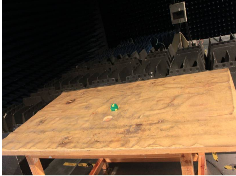
Test frequency above 1GHz at test site 1#
