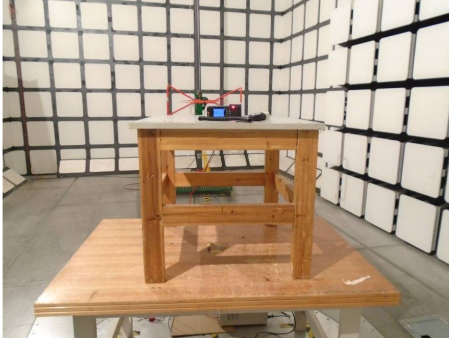
Transmitting Radiated Emissions Front View (Below 1 GHz)
