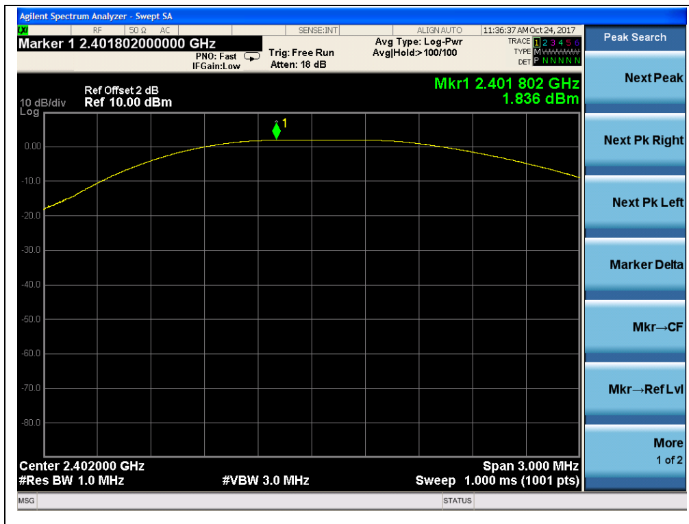
(Channel 0, 2402MHz)
