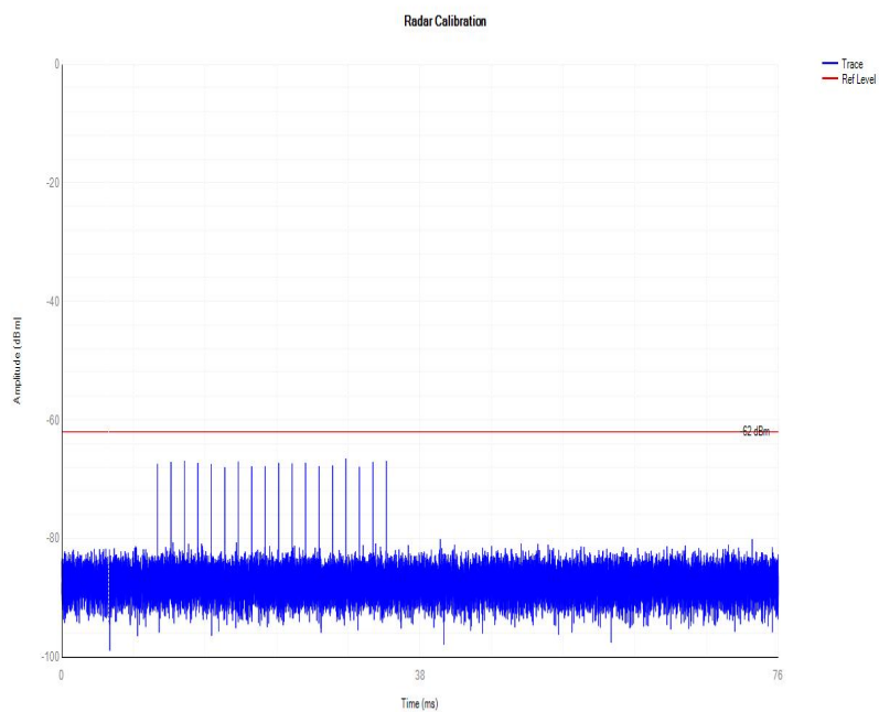
NVNT_ANT1_802_11ac(VHT80)_Calibration_type_0
