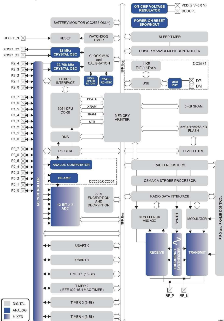
Figure 1-1. CC253x Block Diagram
