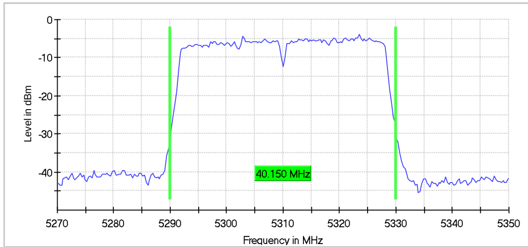
26 dB Bandwidth
