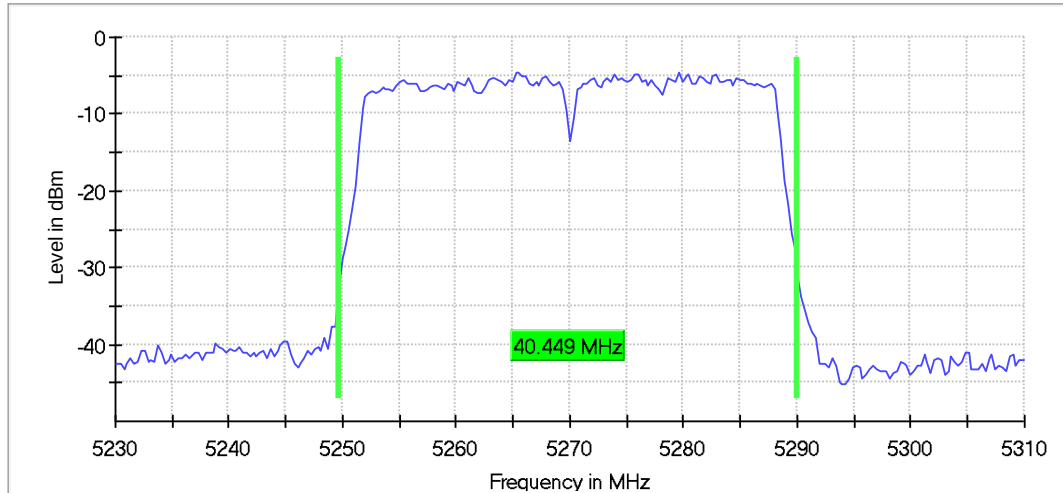
26 dB Bandwidth
