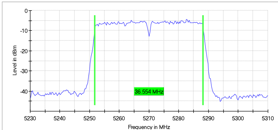
99 %Bandwidth
