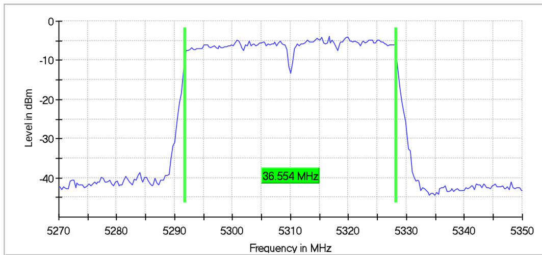
99 %Bandwidth
