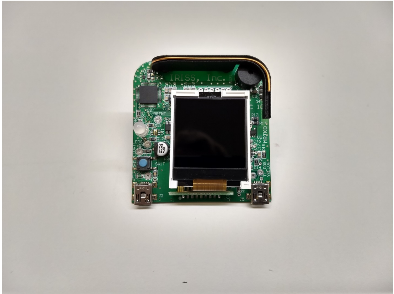
Board – Front
