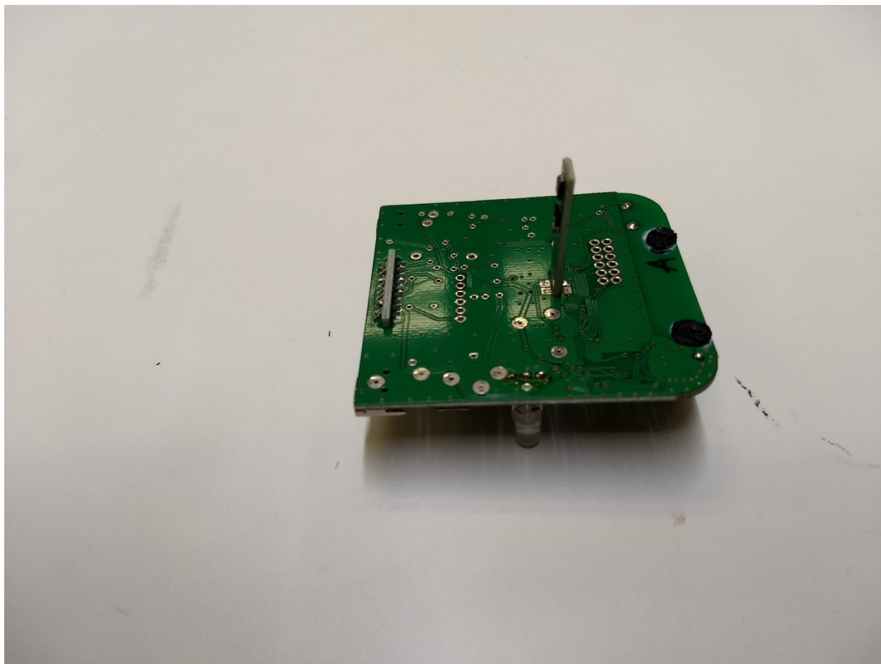
Board Back
