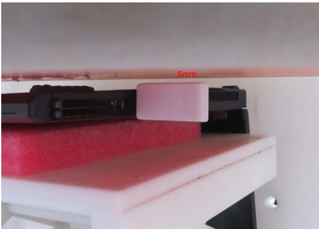
Picture 8: Right Side, the distance from EUT to the bottom of the Phantom is 5mm
