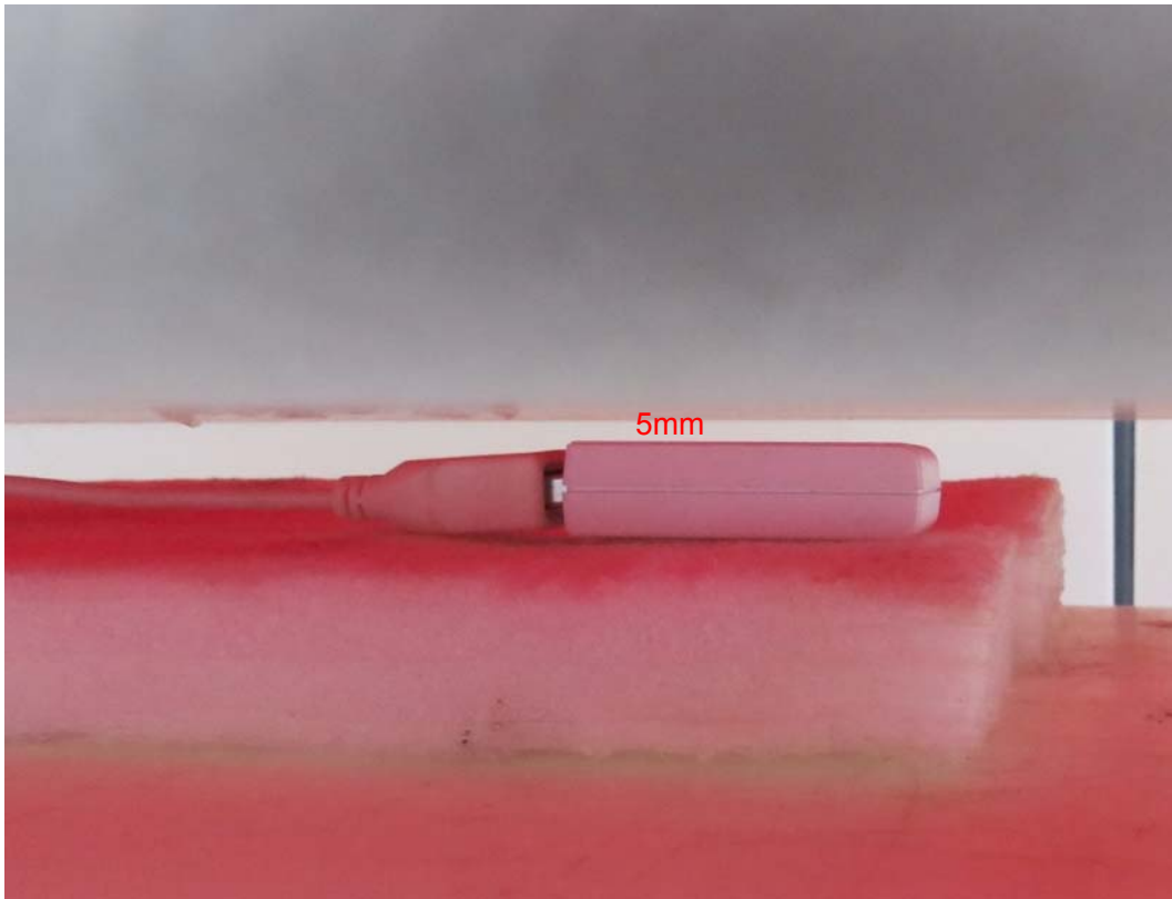
Picture 5: Back Side, the distance from EUT to the bottom of the Phantom is 5mm
