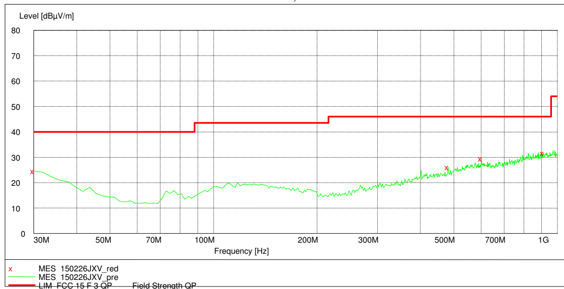
30MHz~1GHz, Horizontal
