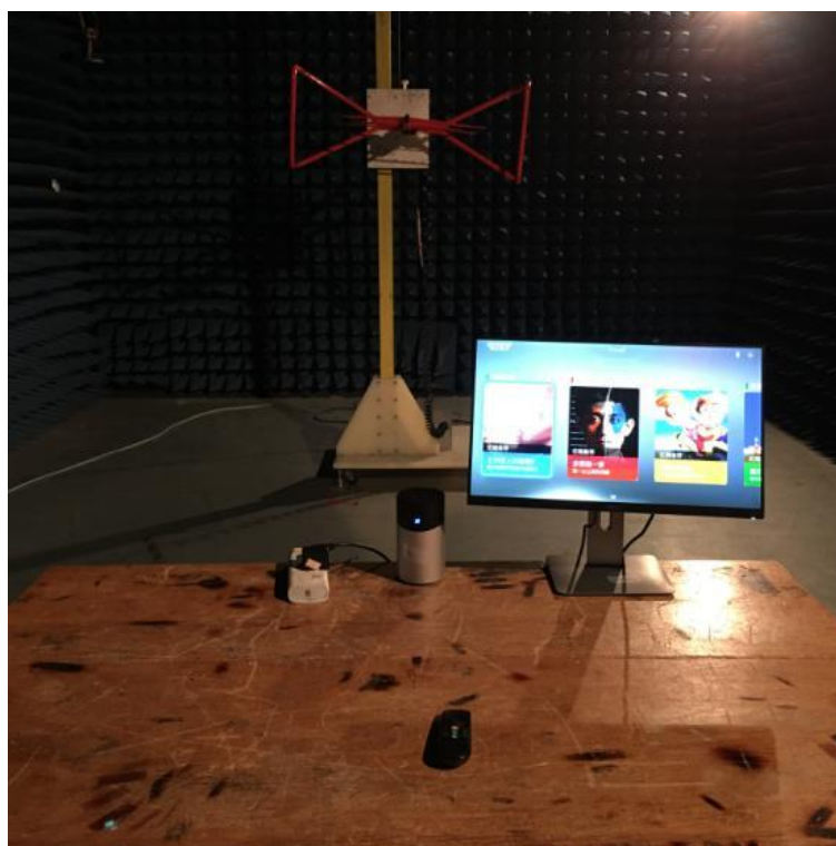
RE TEST SETUP
