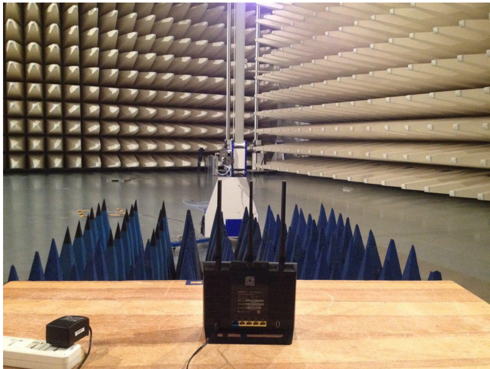
Radiated Emissions
