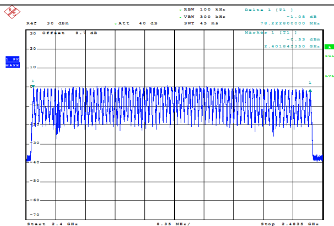
GFSK Modulation
