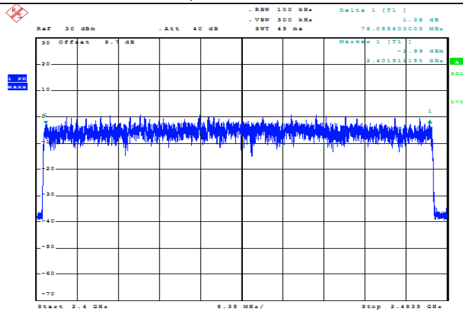
8DPSK Modulation
