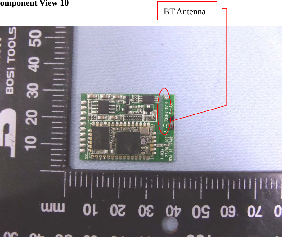
Solder Board-Component View 10
