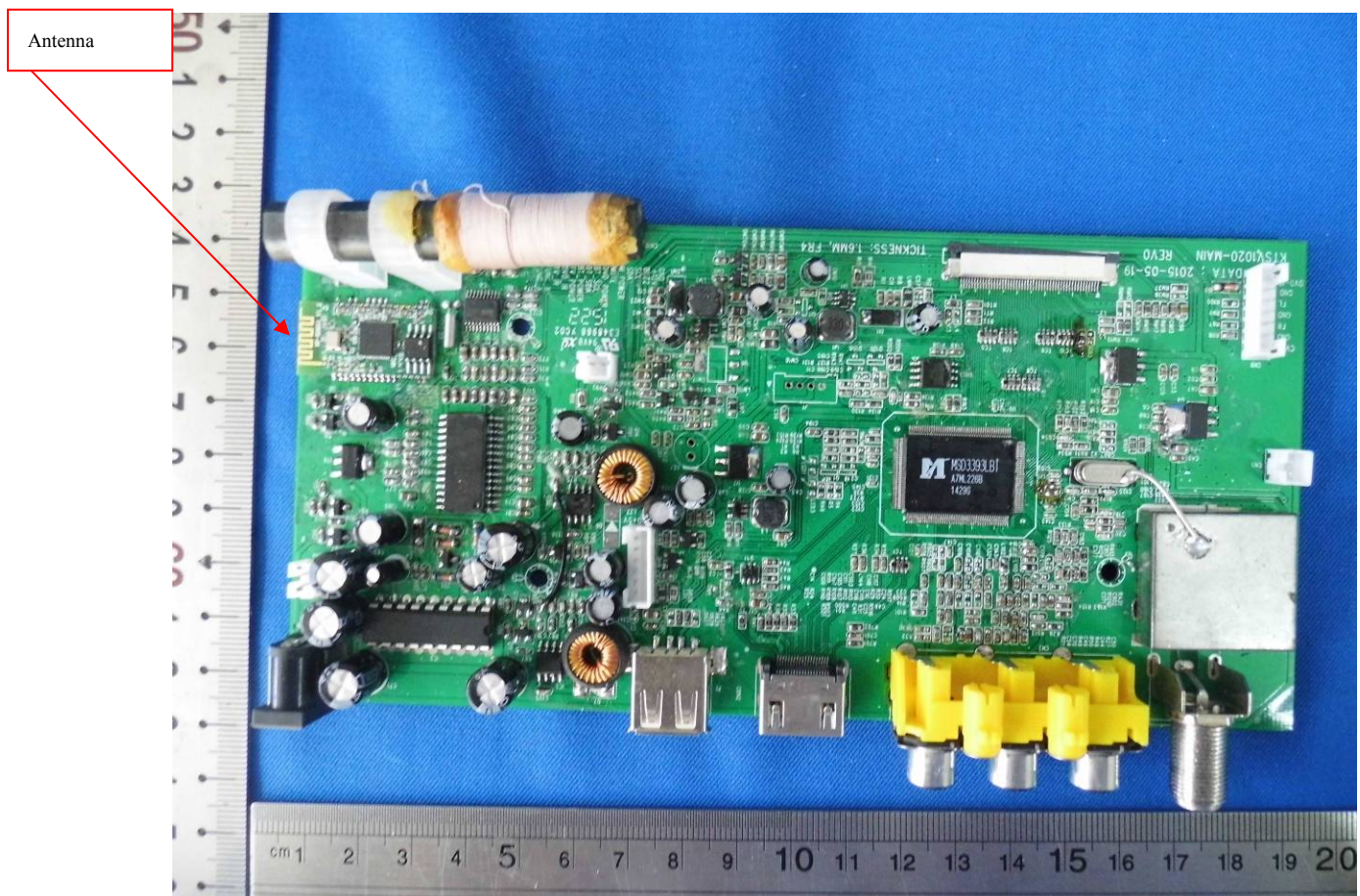
MAIN PCB:
