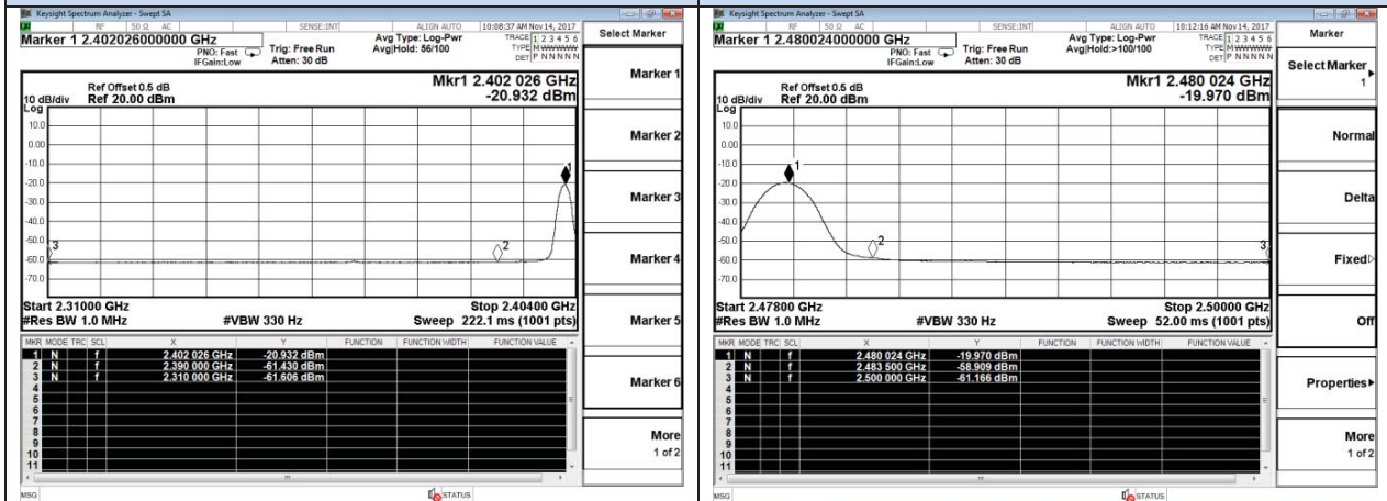
Channel 0 / 2402 MHz - Average
