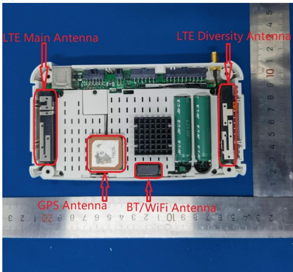
ANT location
