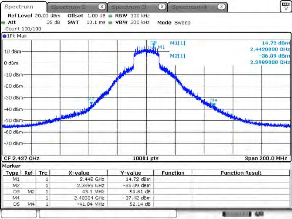
Channel 6 (2437MHz)
