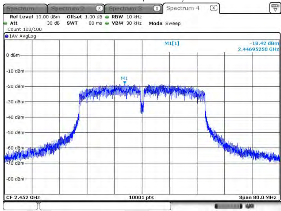
Channel 9 (2452MHz)
