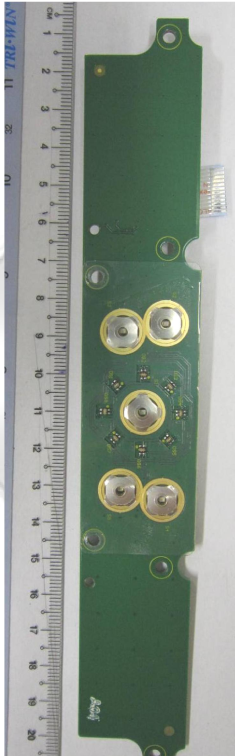
Sub-Board PCB Trace Side
