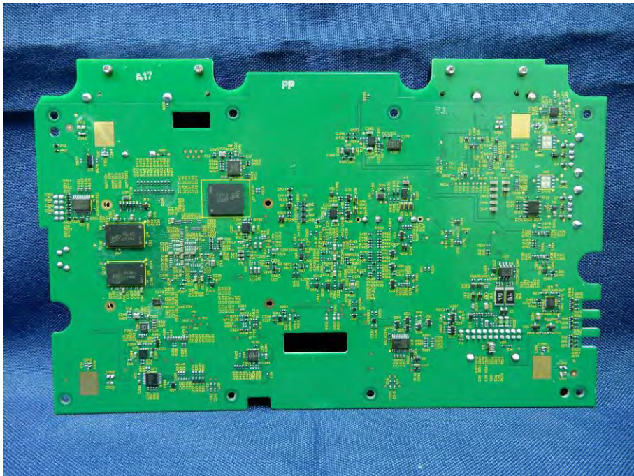
(22) EUT Photo
