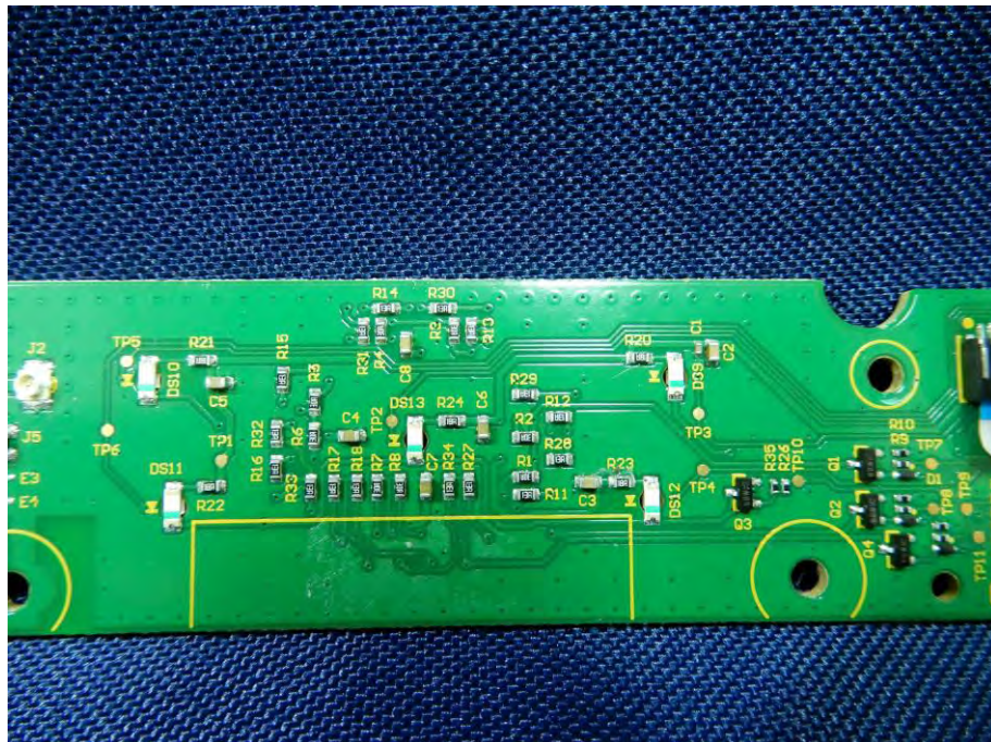
(32) EUT Photo
