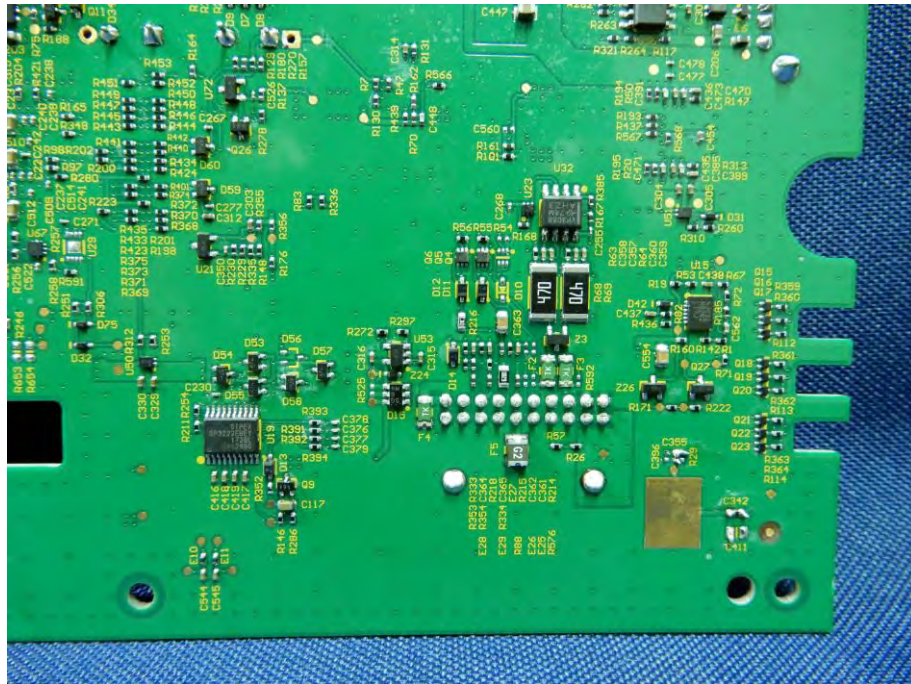
(23) EUT Photo
