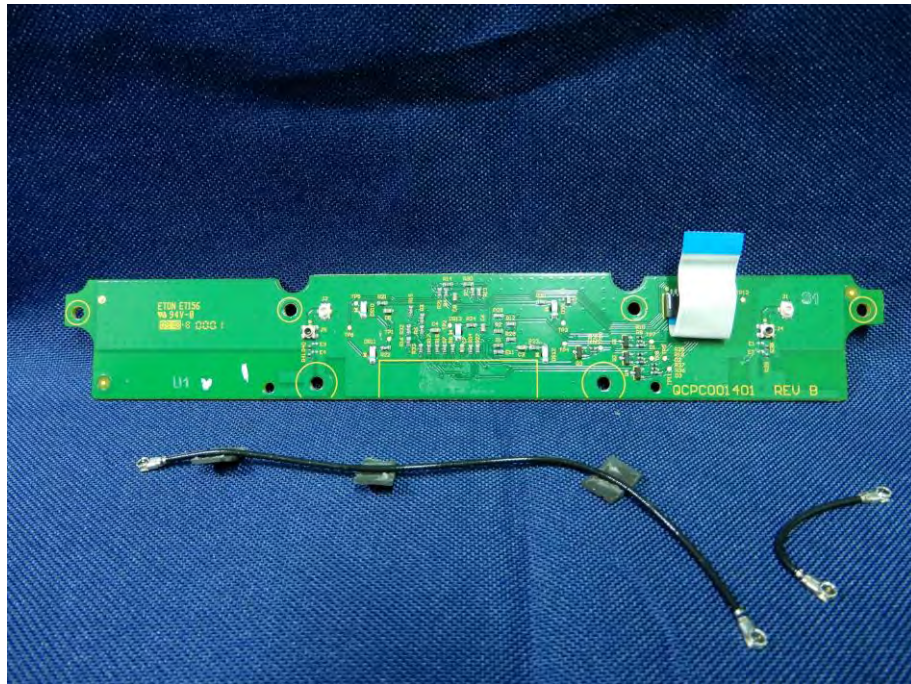
(29) EUT Photo
