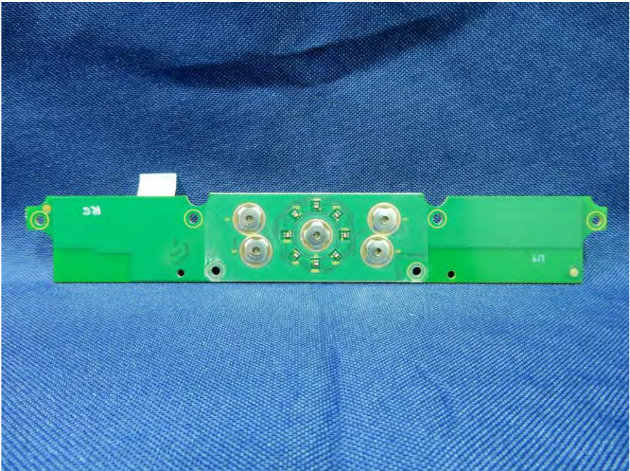
(34) EUT Photo
