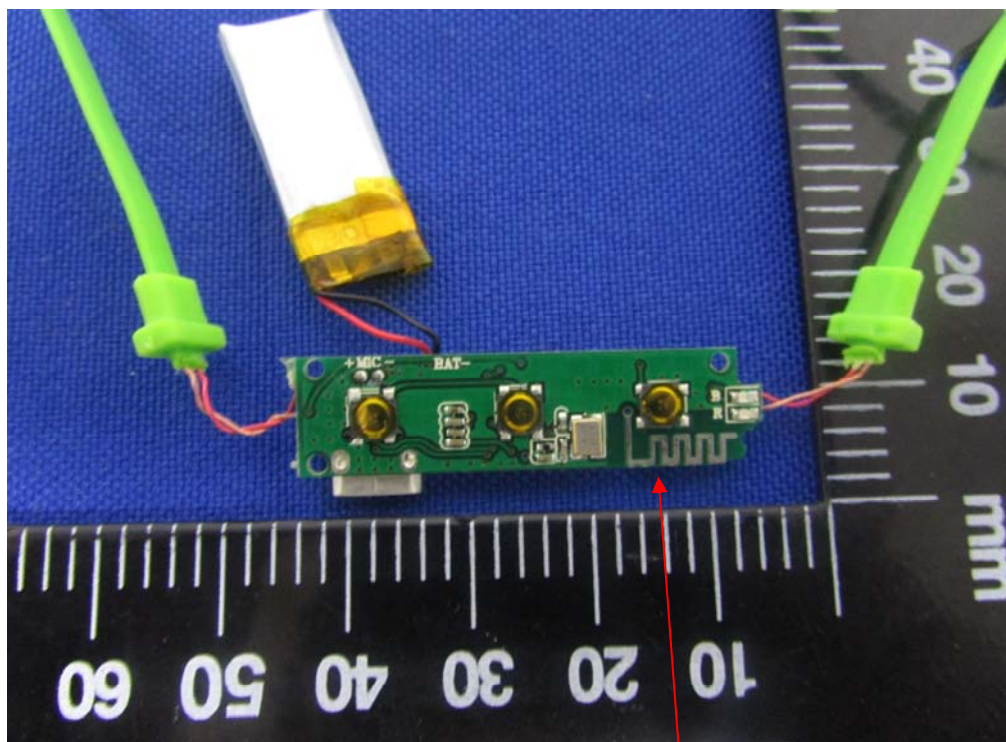
BT Antenna
