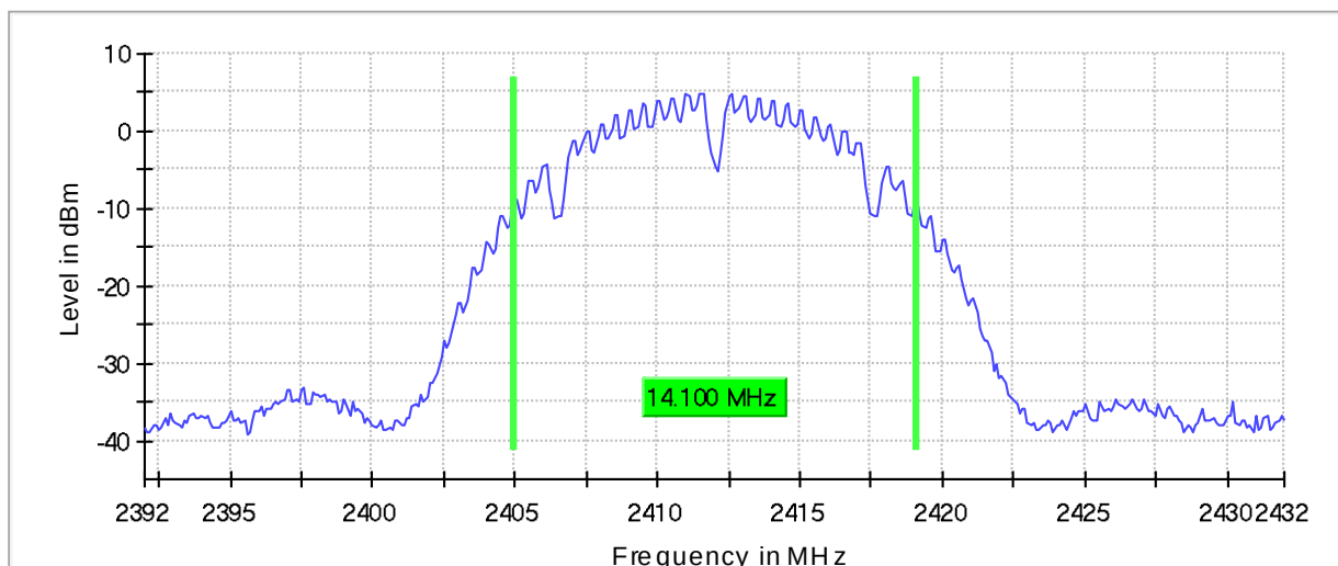
99 %Bandwidth
