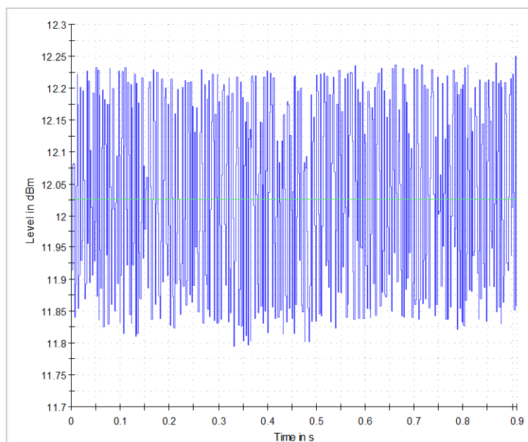
Gated Trace
