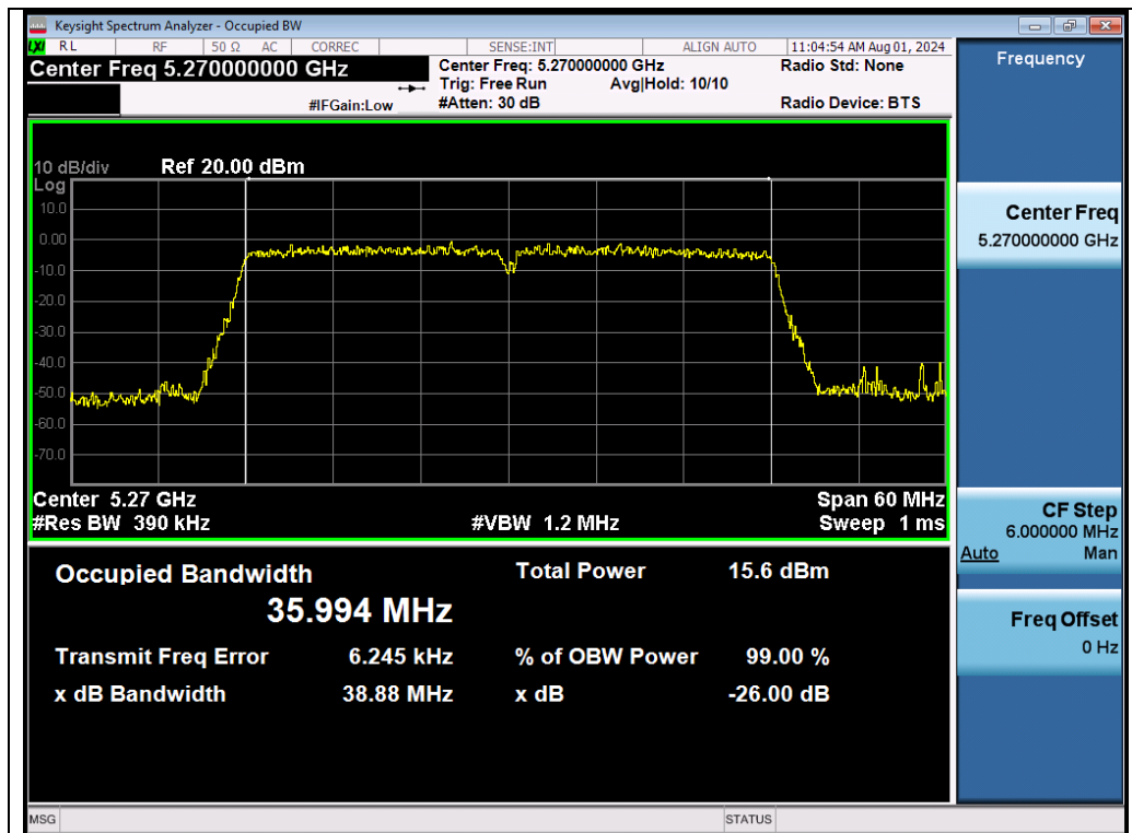
Test_Graph_802.11n40_Chain B_5270_MCS0_OBW
