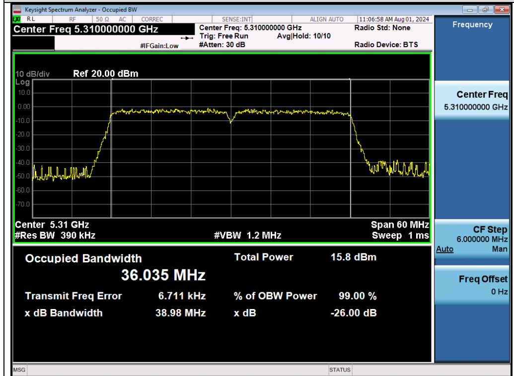
Test_Graph_802.11n40_Chain B_5310_MCS0_OBW
