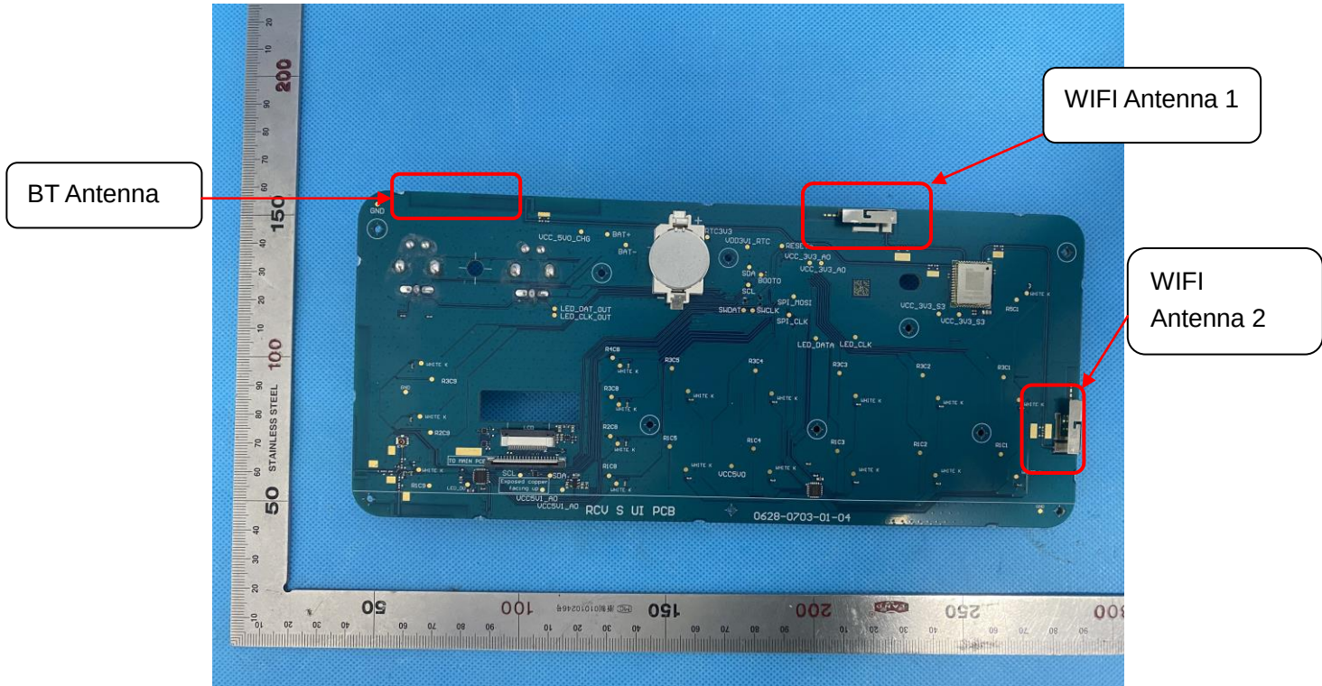
Internal View-2 of EUT
