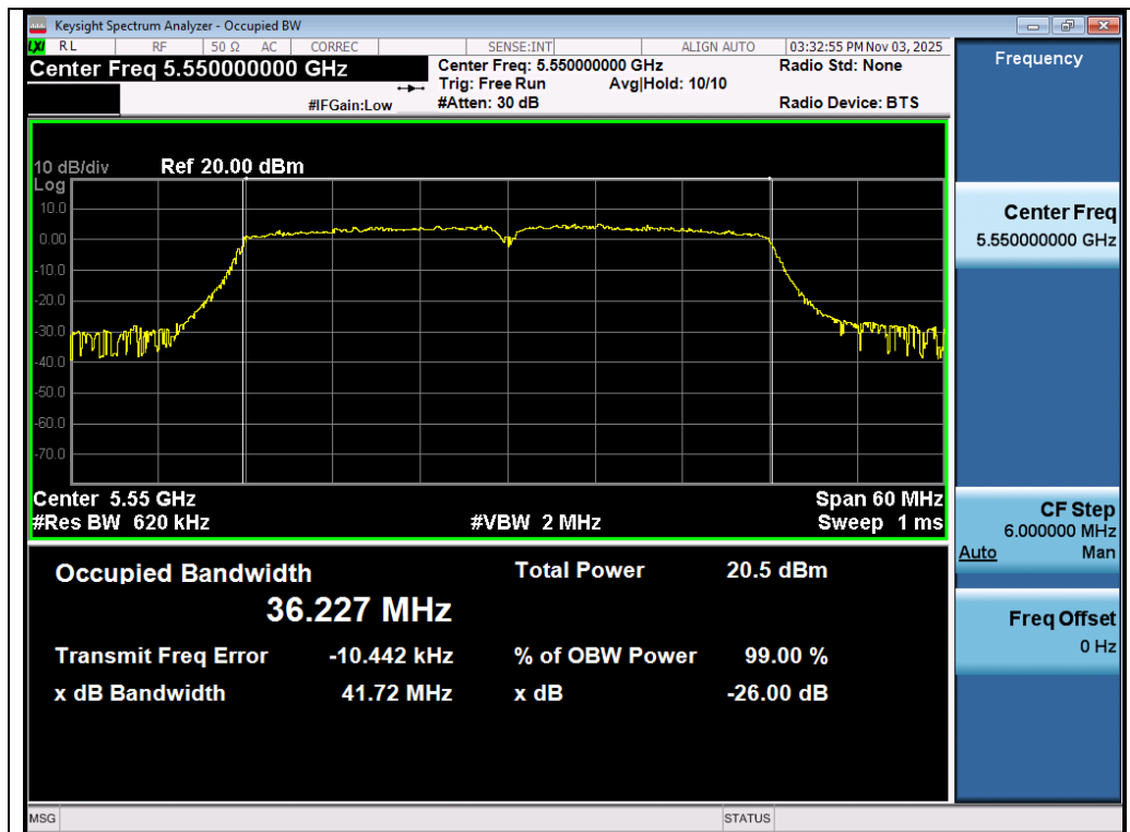
Test_Graph_802.11n40_Ant 2_5550_MCS0_OBW
