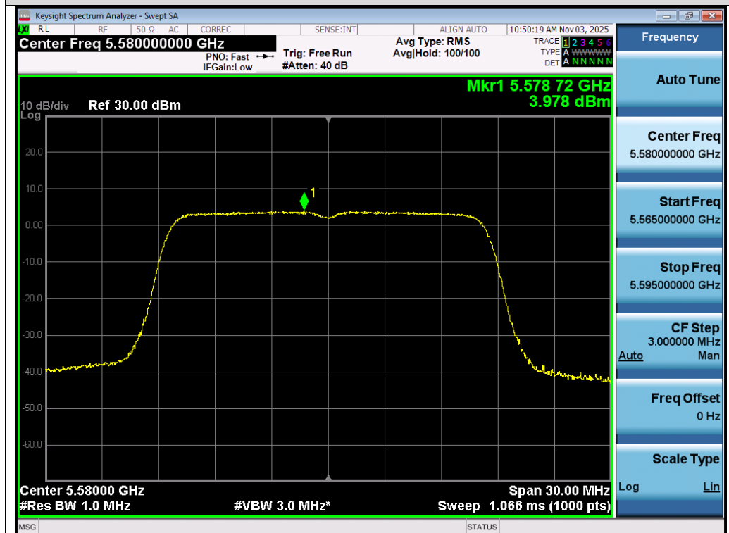
Test_Graph_802.11a_Ant 1_5580_6Mbps_PSD
