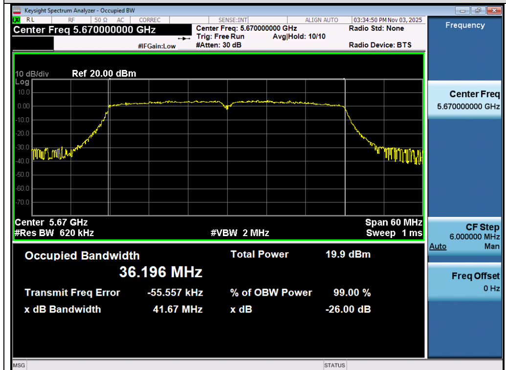
Test_Graph_802.11n40_Ant 2_5670_MCS0_OBW
