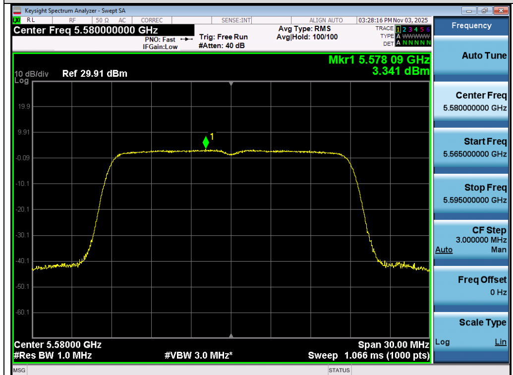
Test_Graph_802.11n20_Ant 2_5580_MCS0_PSD
