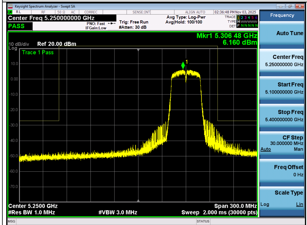
Test_Graph_802.11n40_Ant 2_5310_MCS0_Frequency Band 3
