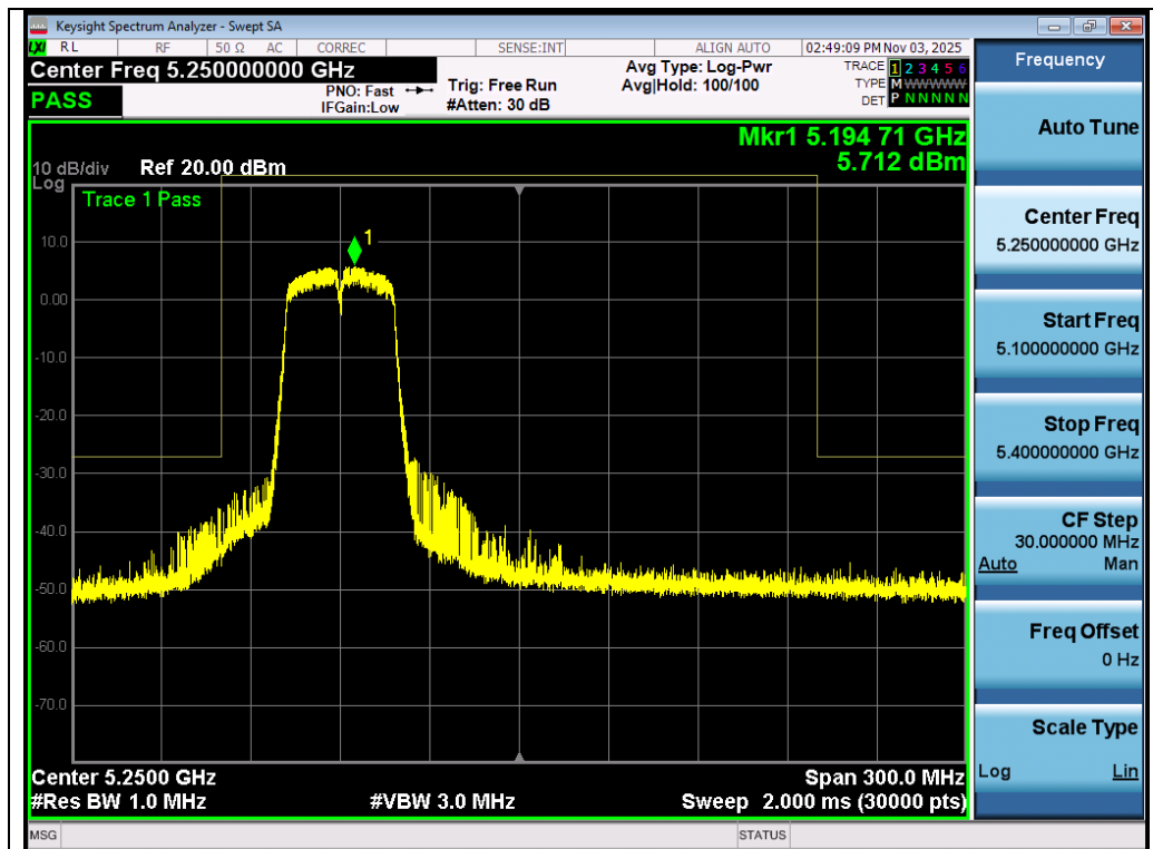
Test_Graph_802.11n40_Ant 2_5190_MCS0_Frequency Band 3
