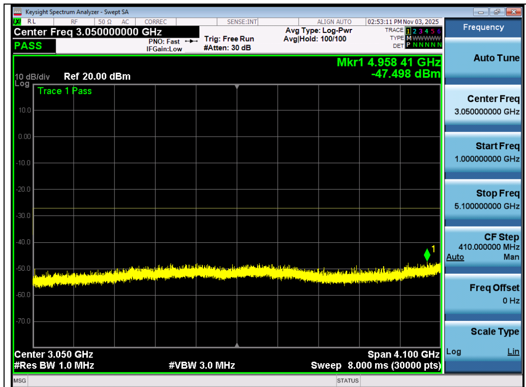
Test_Graph_802.11n40_Ant 2_5230_MCS0_Frequency Band 2
