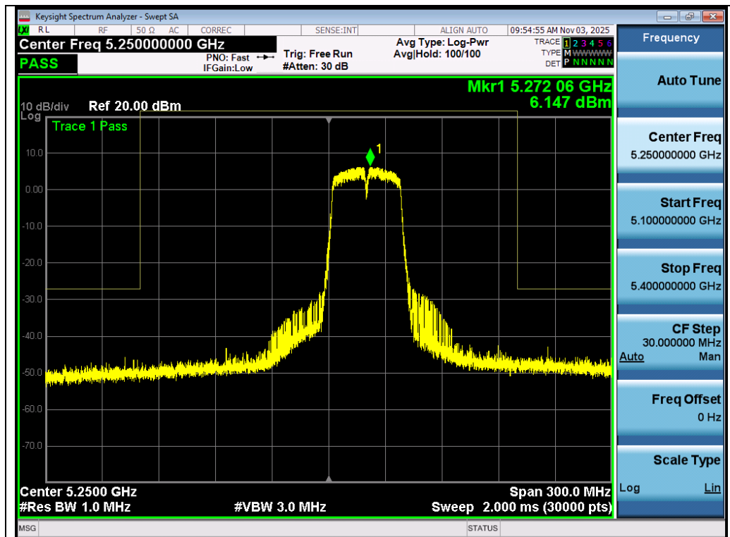
Test_Graph_802.11n40_Ant 1_5270_MCS0_Frequency Band 3
