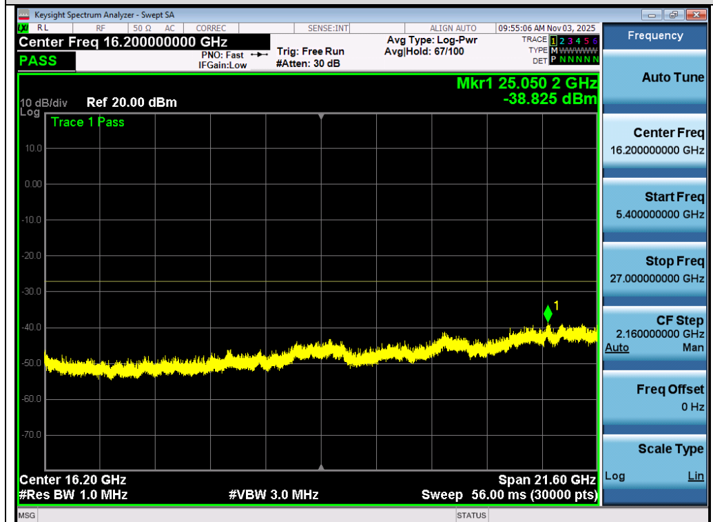
Test_Graph_802.11n40_Ant 1_5270_MCS0_Frequency Band 4
