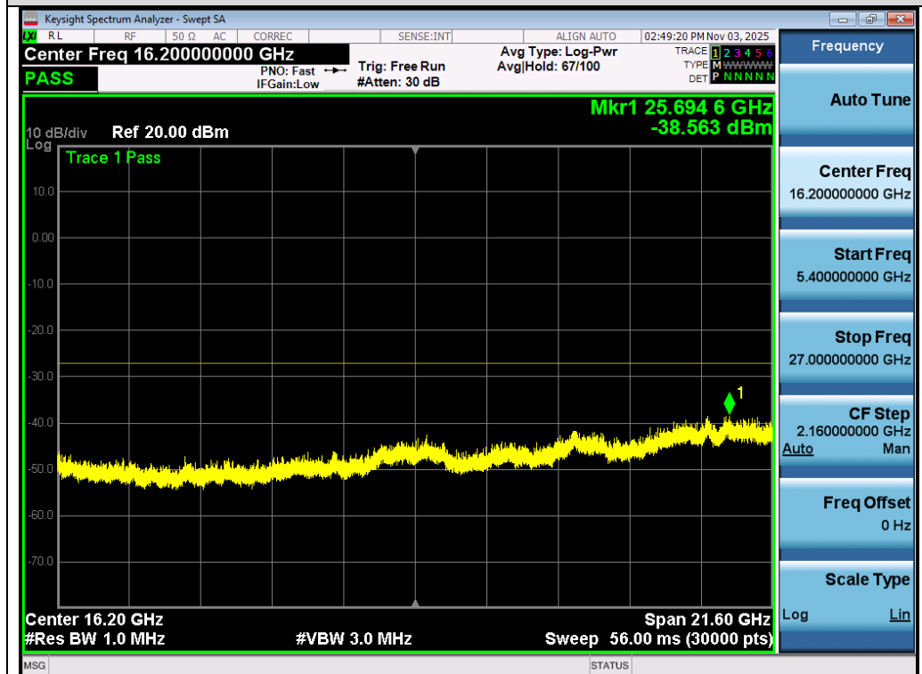
Test_Graph_802.11n40_Ant 2_5190_MCS0_Frequency Band 4
