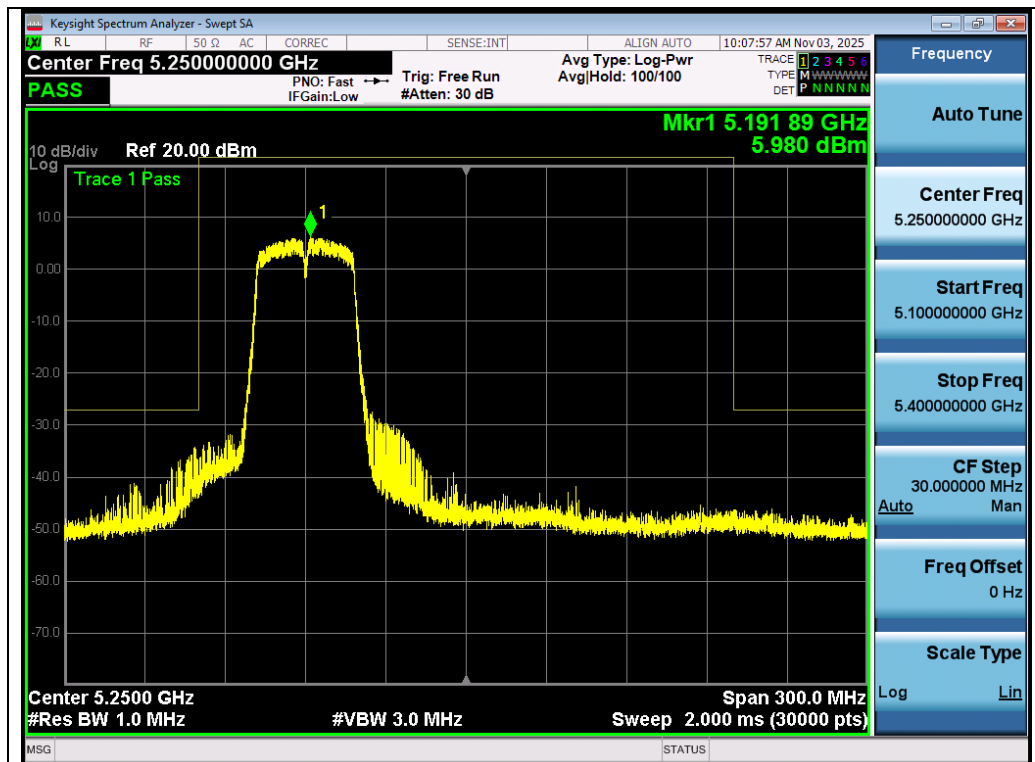
Test_Graph_802.11n40_Ant 1_5190_MCS0_Frequency Band 3
