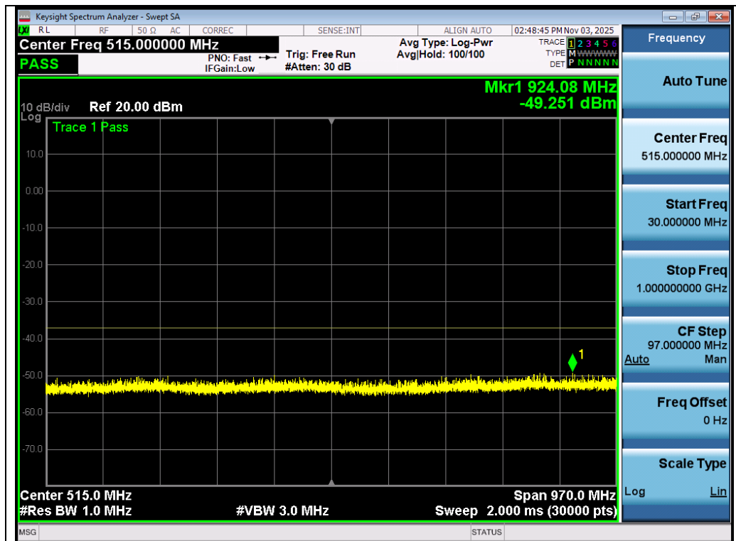
Test_Graph_802.11n40_Ant 2_5190_MCS0_Frequency Band 1
