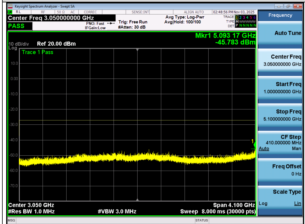
Test_Graph_802.11n40_Ant 2_5190_MCS0_Frequency Band 2
