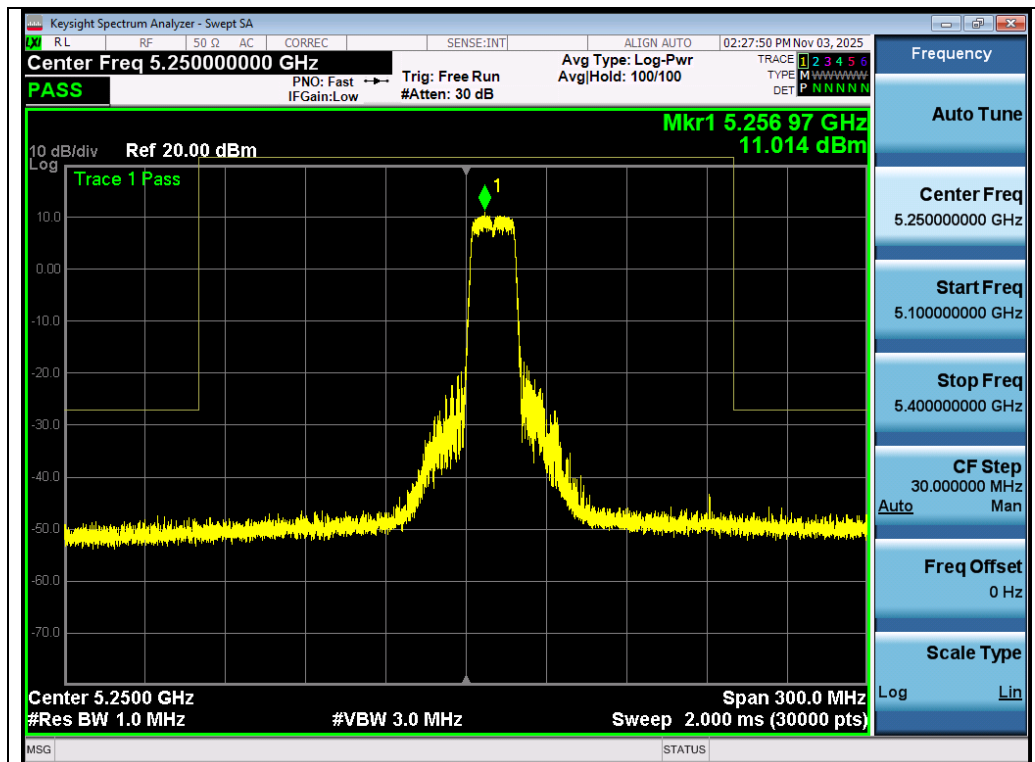
Test_Graph_802.11a_Ant 2_5260_6Mbps_Frequency Band 3
