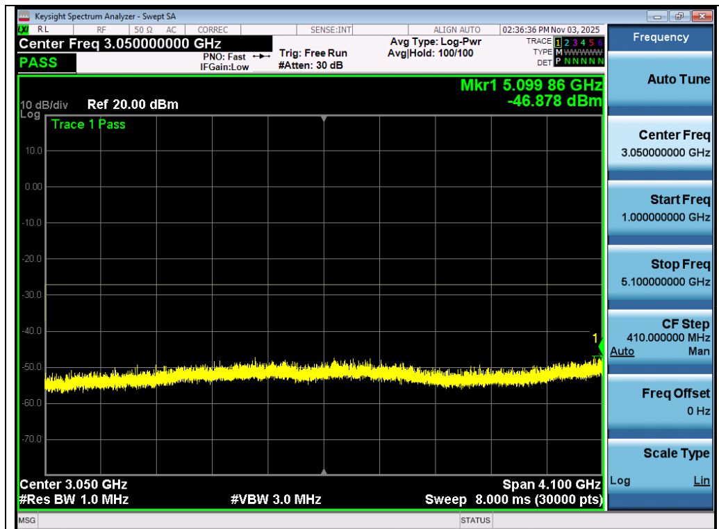
Test_Graph_802.11n40_Ant 2_5310_MCS0_Frequency Band 2
