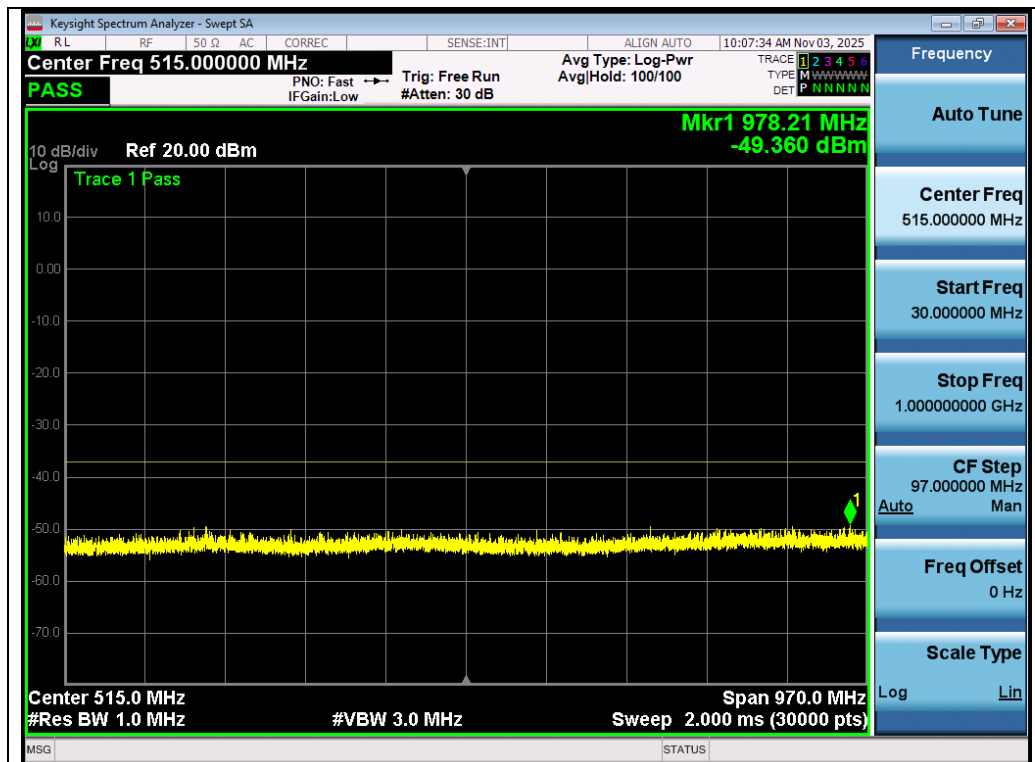
Test_Graph_802.11n40_Ant 1_5190_MCS0_Frequency Band 1
