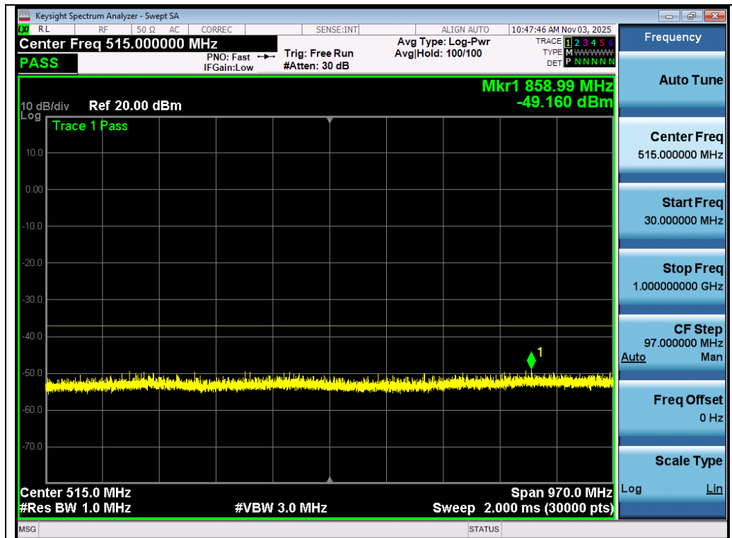
Test_Graph_802.11a_Ant 1_5500_6Mbps_Frequency Band 1
