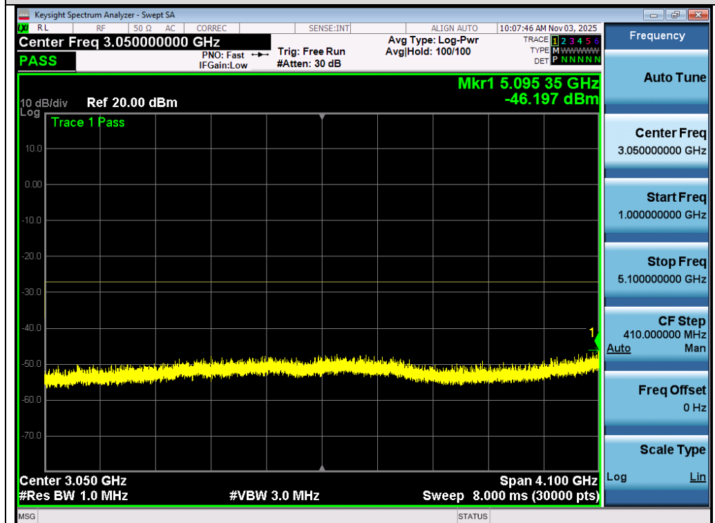
Test_Graph_802.11n40_Ant 1_5190_MCS0_Frequency Band 2
