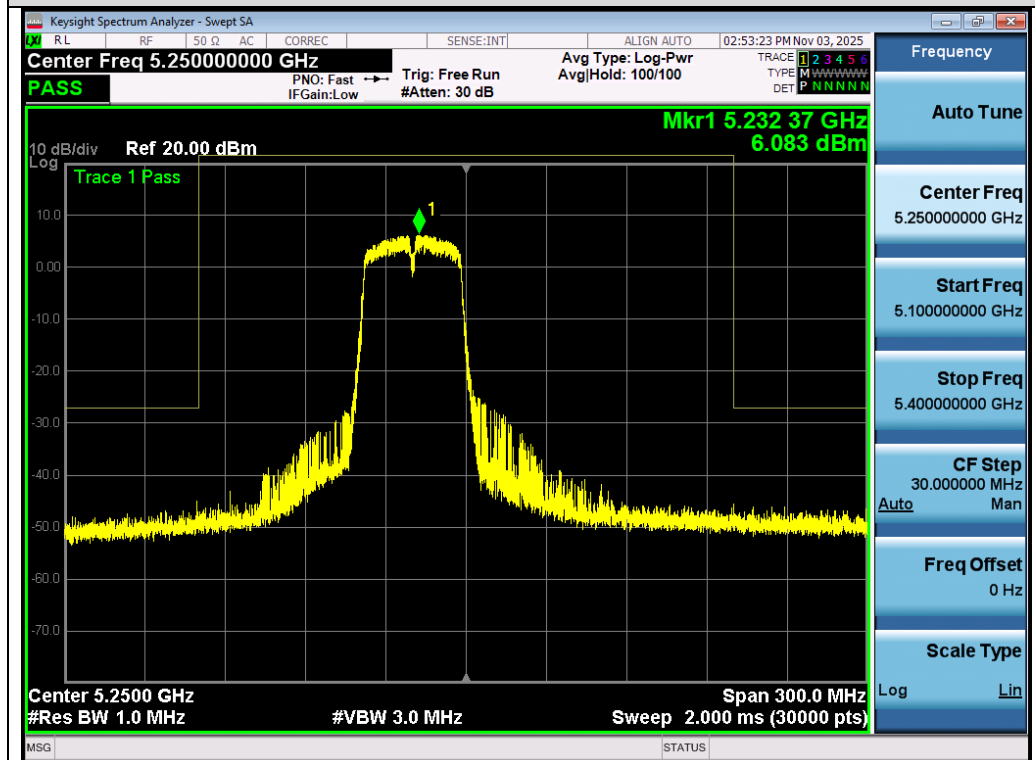
Test_Graph_802.11n40_Ant 2_5230_MCS0_Frequency Band 3
