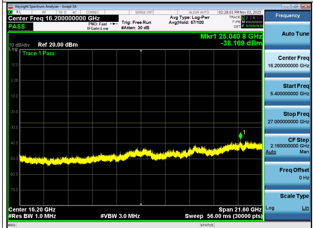
Test_Graph_802.11a_Ant 2_5260_6Mbps_Frequency Band 4
