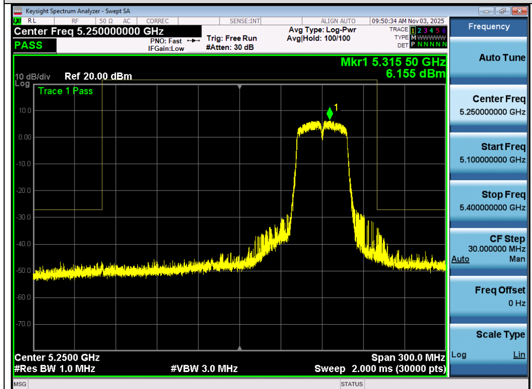
Test_Graph_802.11n40_Ant 1_5310_MCS0_Frequency Band 3
