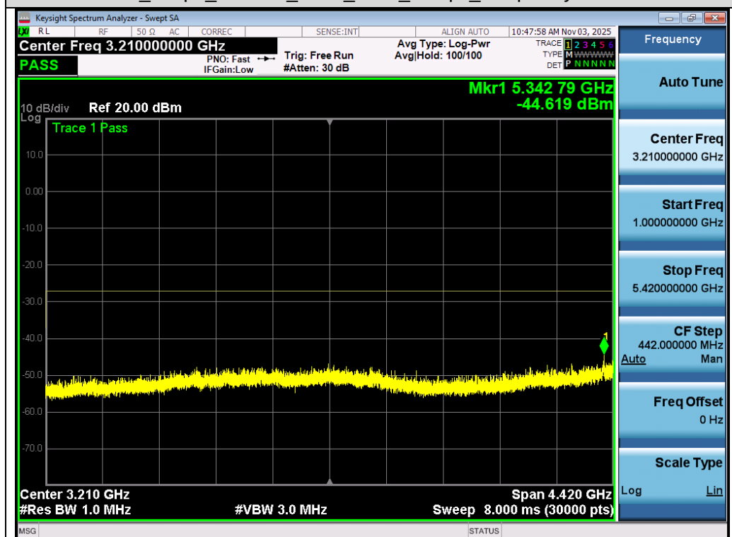
Test_Graph_802.11a_Ant 1_5500_6Mbps_Frequency Band 2
