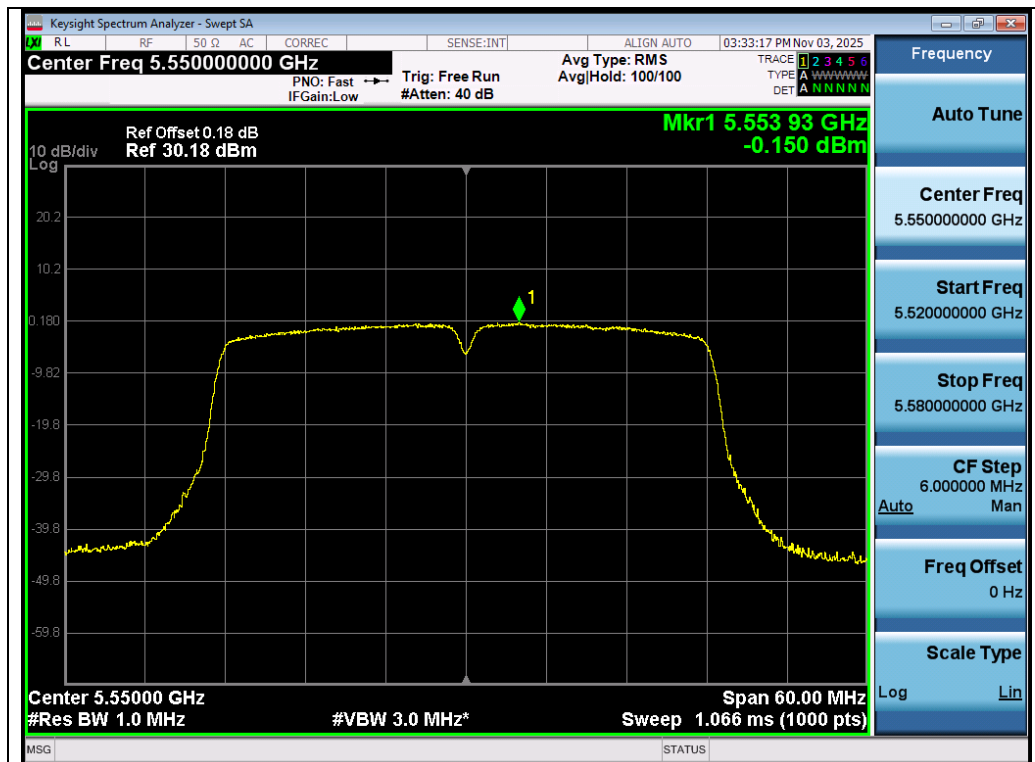
Test_Graph_802.11n40_Ant 2_5550_MCS0_PSD
