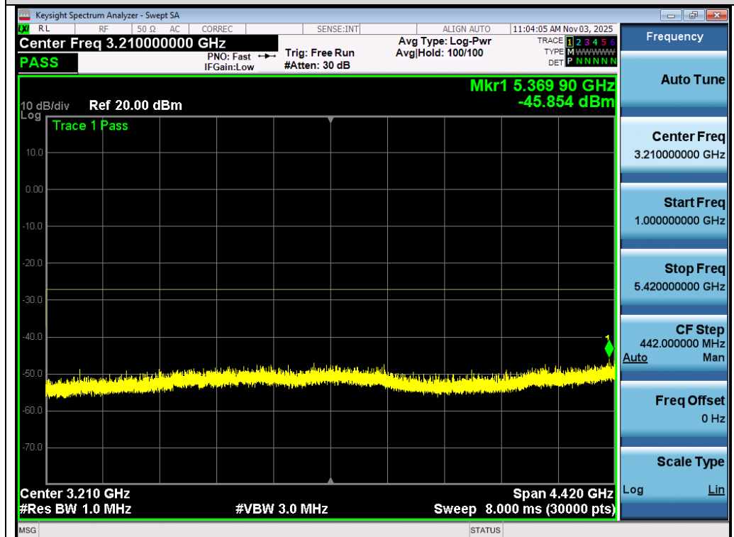
Test_Graph_802.11n40_Ant 1_5670_MCS0_Frequency Band 2
