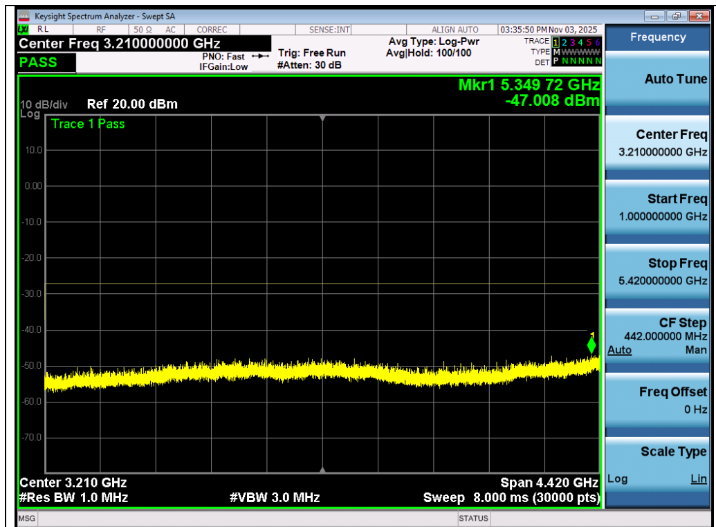
Test_Graph_802.11n40_Ant 2_5670_MCS0_Frequency Band 2
