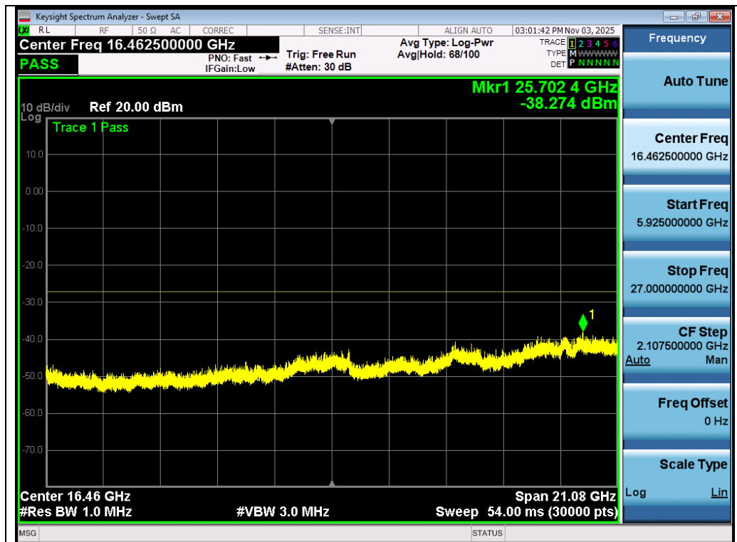
Test_Graph_802.11a_Ant 2_5825_6Mbps_Frequency Band4
