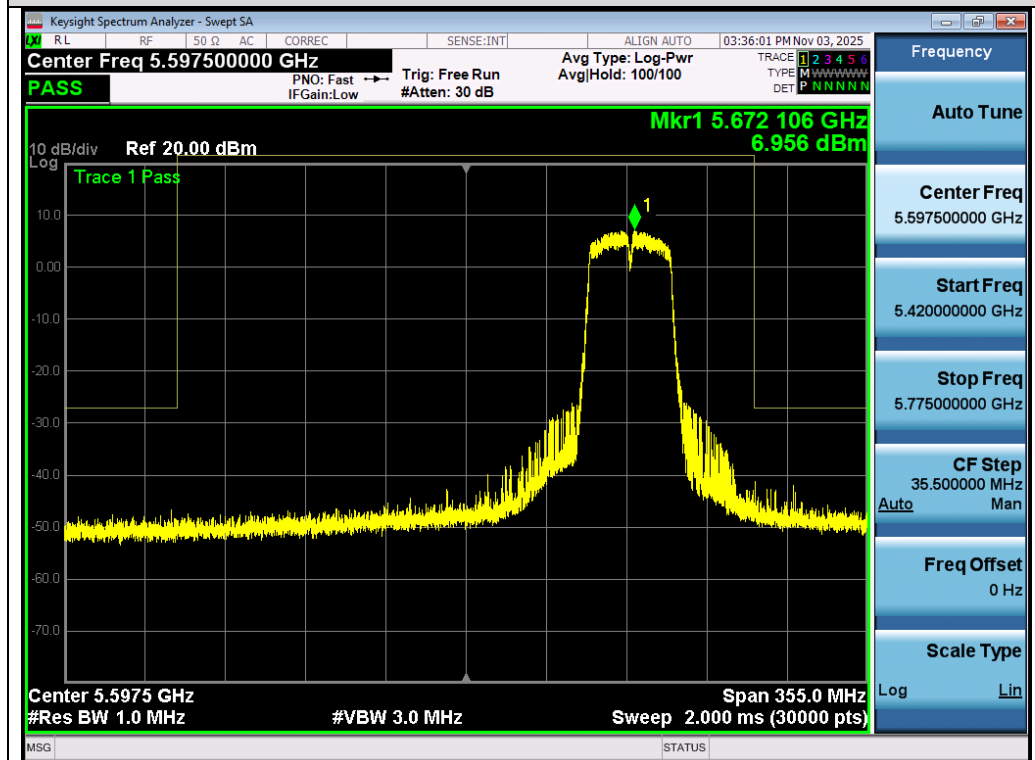
Test_Graph_802.11n40_Ant 2_5670_MCS0_Frequency Band 3
