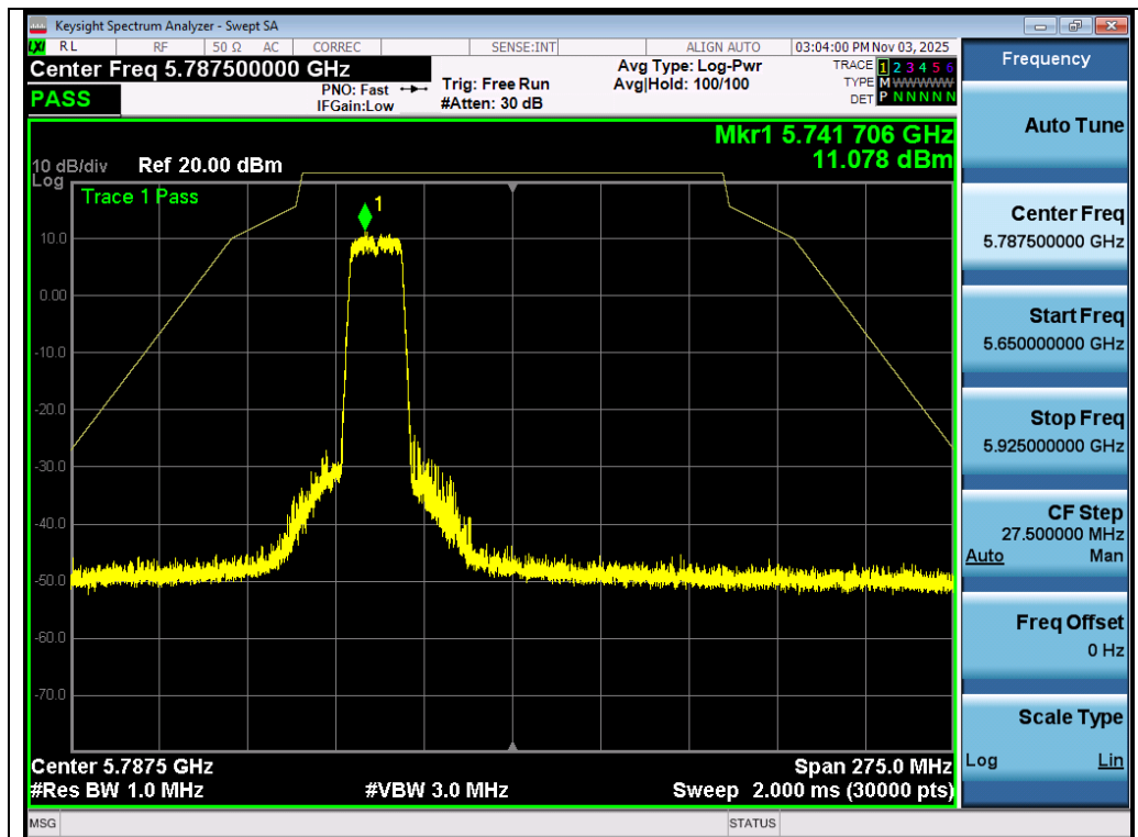
Test_Graph_802.11a_Ant 2_5745_6Mbps_Frequency Band3
