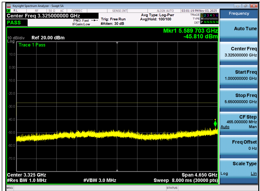
Test_Graph_802.11a_Ant 2_5825_6Mbps_Frequency Band2
