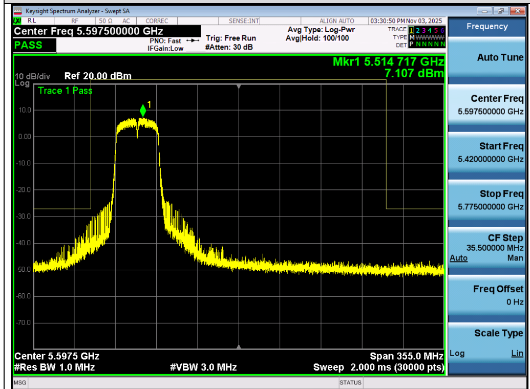
Test_Graph_802.11n40_Ant 2_5510_MCS0_Frequency Band 3
