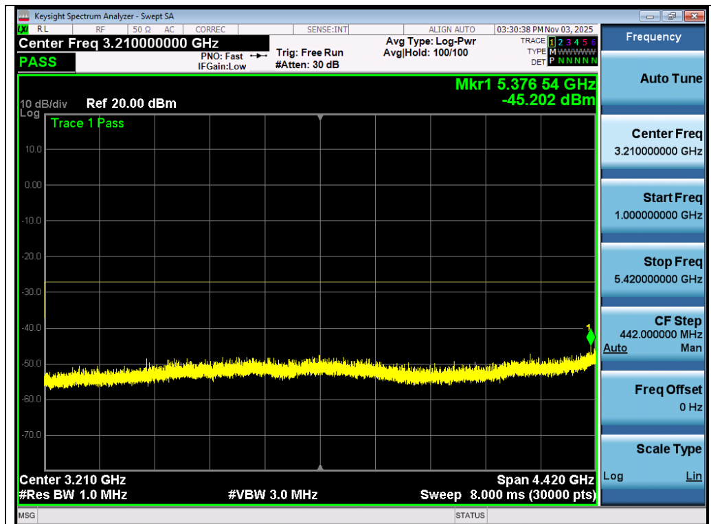
Test_Graph_802.11n40_Ant 2_5510_MCS0_Frequency Band 2
