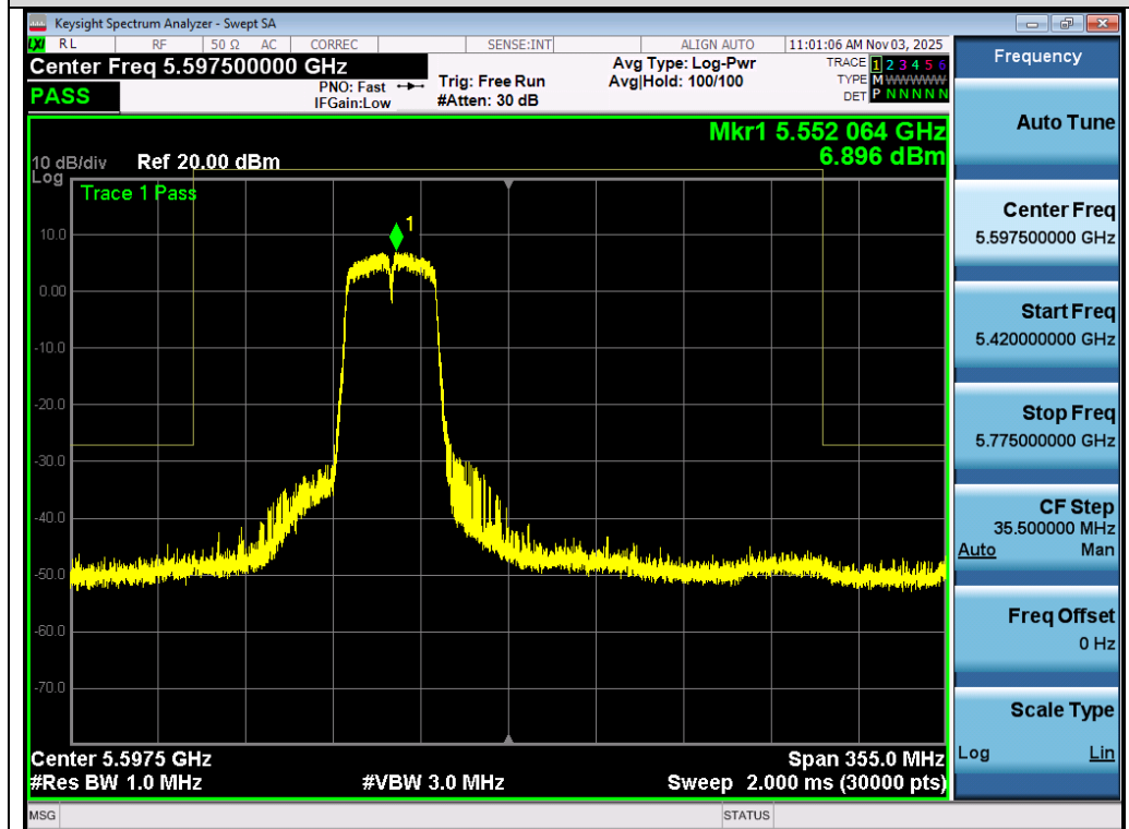
Test_Graph_802.11n40_Ant 1_5550_MCS0_Frequency Band 3
