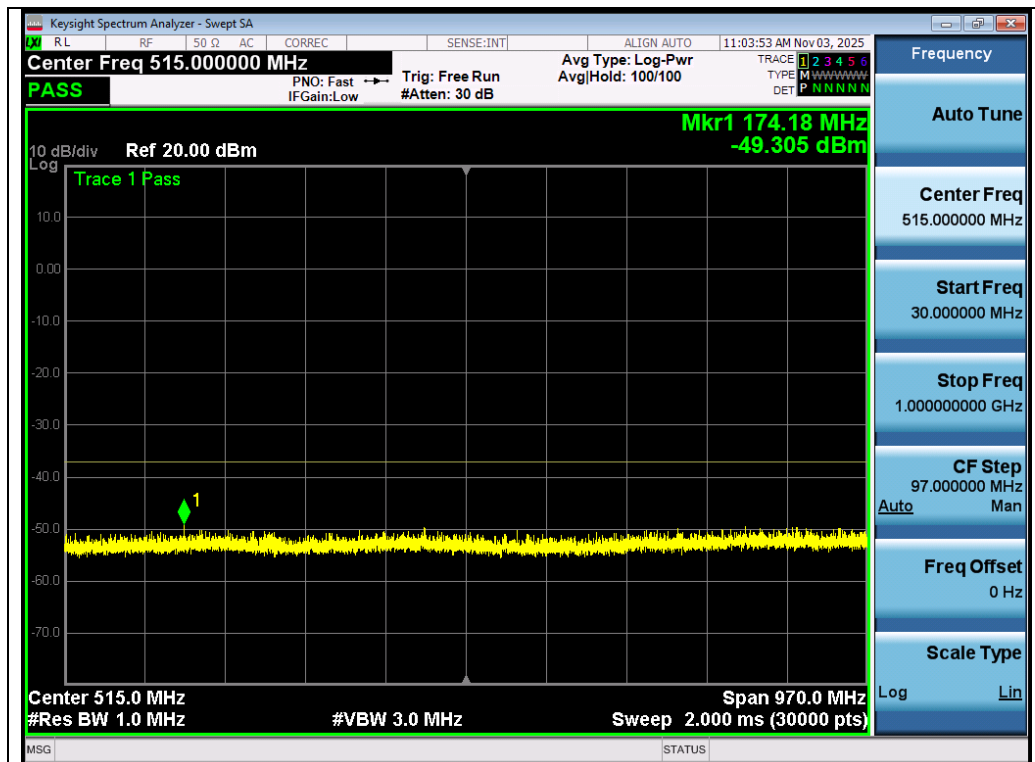
Test_Graph_802.11n40_Ant 1_5670_MCS0_Frequency Band 1
