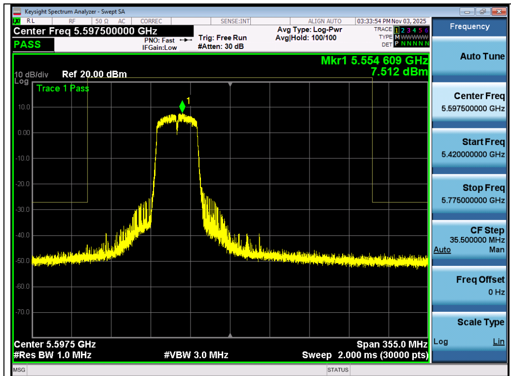
Test_Graph_802.11n40_Ant 2_5550_MCS0_Frequency Band 3
