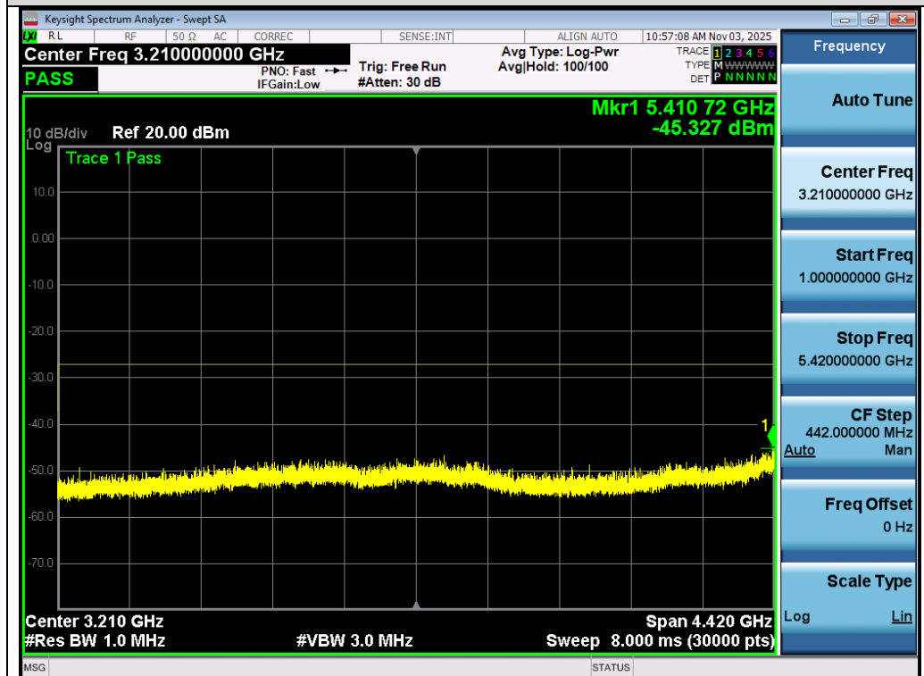
Test_Graph_802.11n40_Ant 1_5510_MCS0_Frequency Band 2
