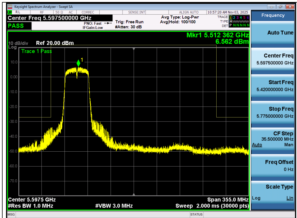
Test_Graph_802.11n40_Ant 1_5510_MCS0_Frequency Band 3
