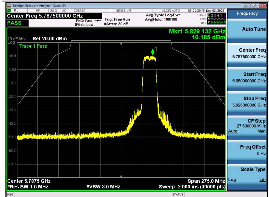
Test_Graph_802.11a_Ant 2_5825_6Mbps_Frequency Band3
