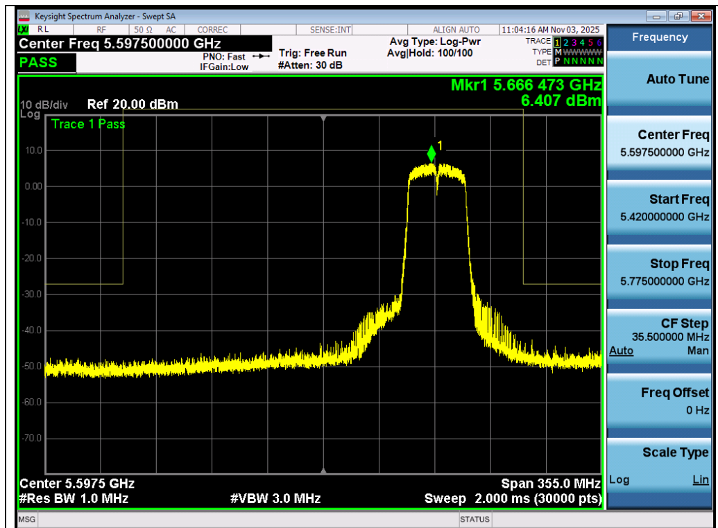
Test_Graph_802.11n40_Ant 1_5670_MCS0_Frequency Band 3
