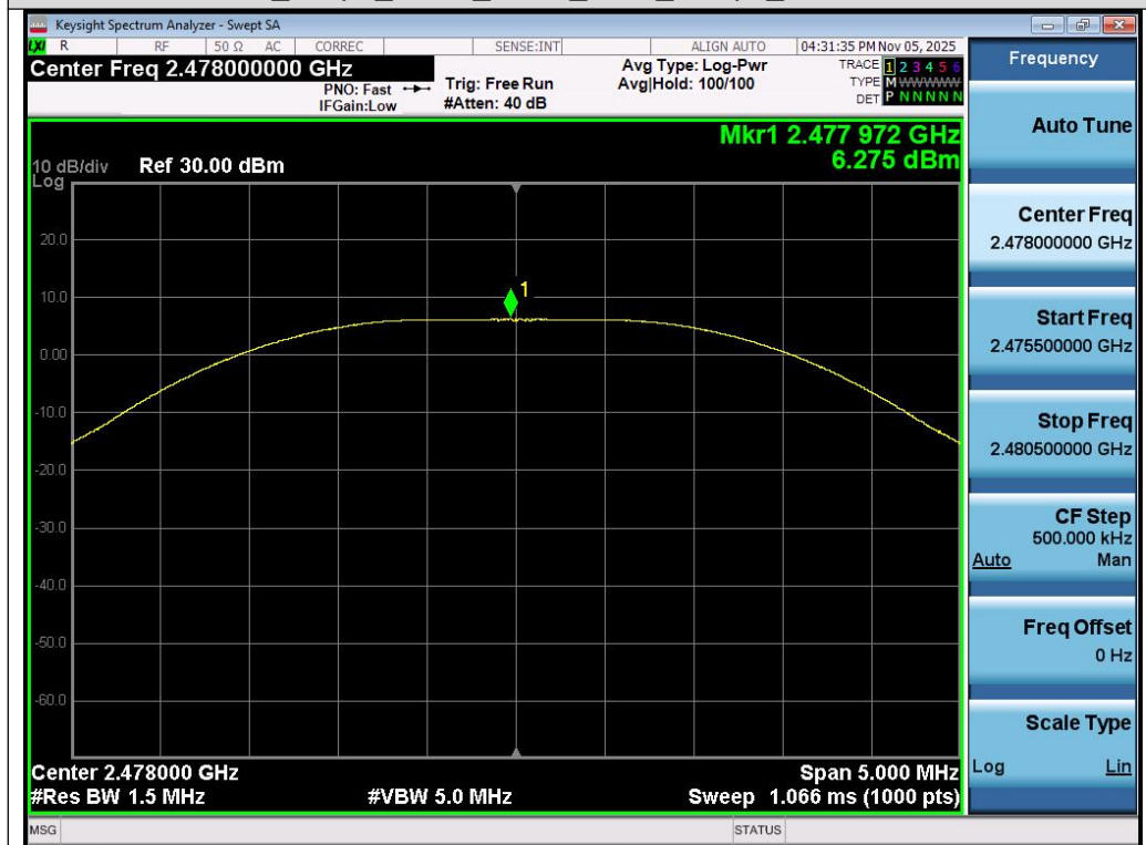
Test_Graph_LE2M_ANT1_2478_2Mbps_Peak Power
