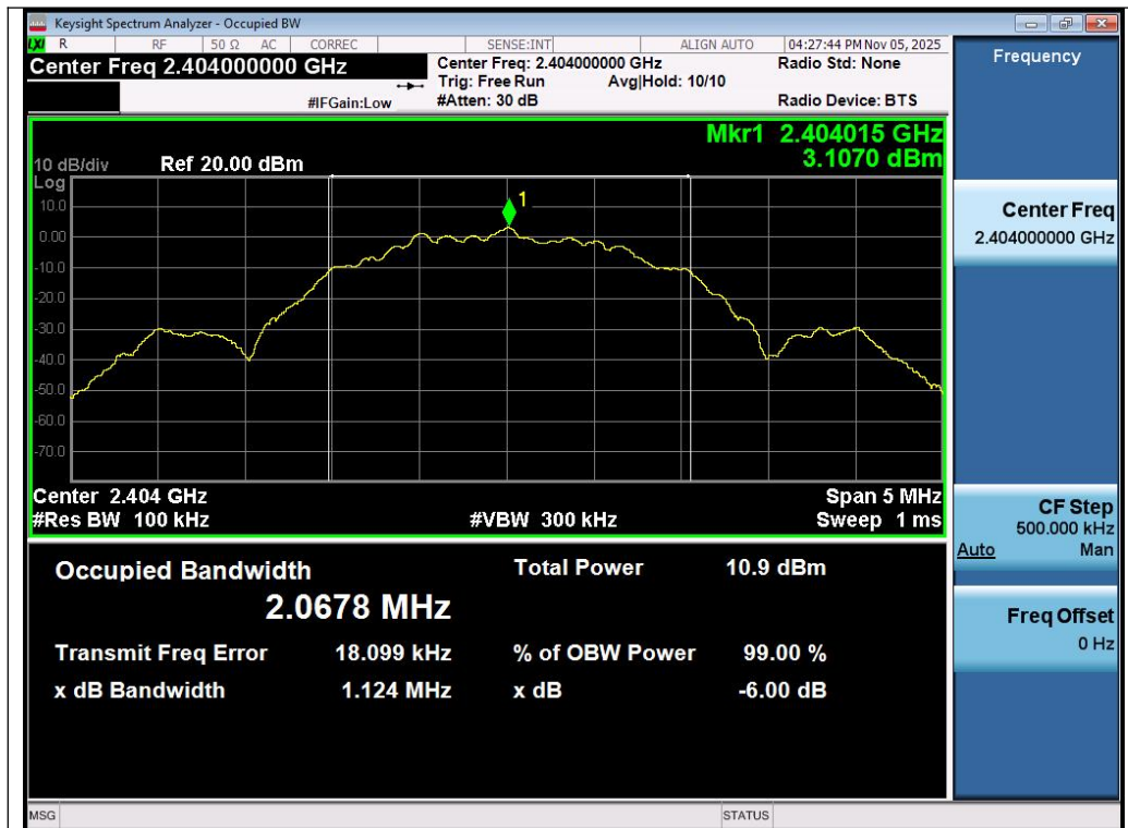
Test_Graph_LE2M_ANT1_2404_2Mbps_DTSBW
