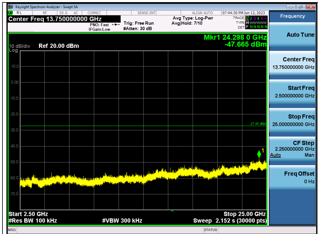
Test_Graph_ANT1_2480_Higher Band Emissions
