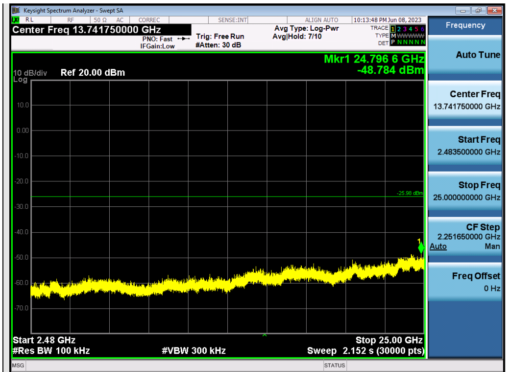
Test_Graph_ANT2_2440_Higher Band Emissions
