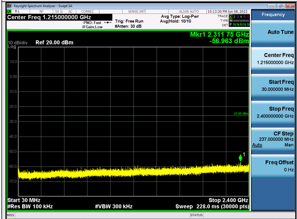
Test_Graph_ANT2_2440_Lower Band Emissions
