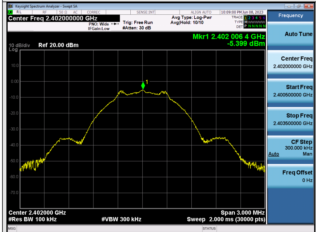
Test_Graph_ANT2_2402_Reference Level
