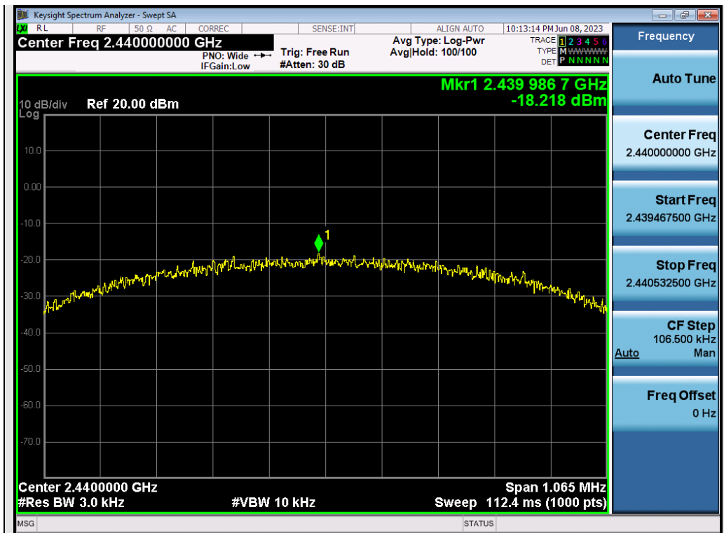
Test_Graph_ANT2_2440_PSD
