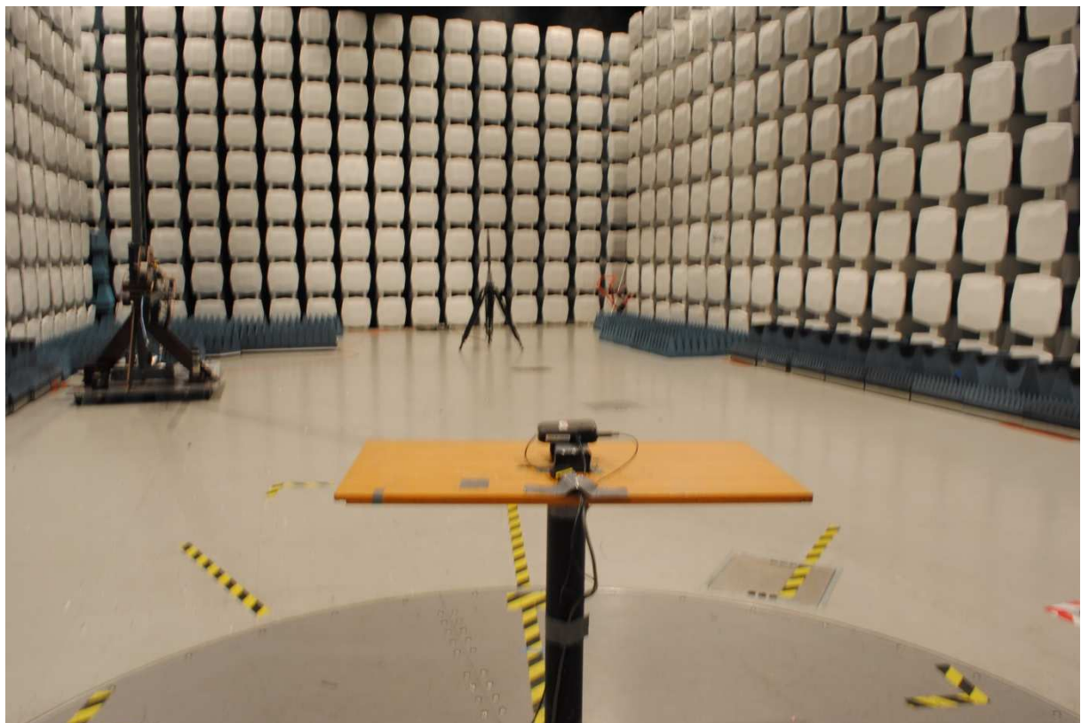
Radiated Emissions, Less than 30MHz, 10m
