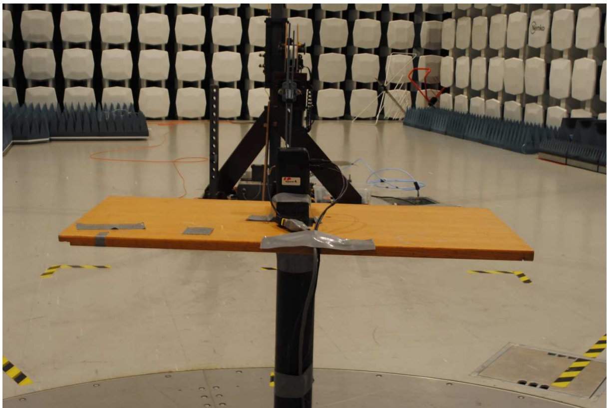
Radiated Emissions, 30 - 1000 MHz, 3m
