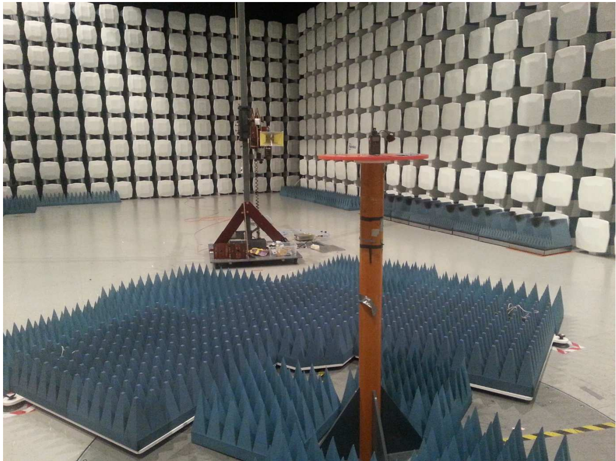
Radiated Emissions, 1 – 8.5 GHz, @3m
