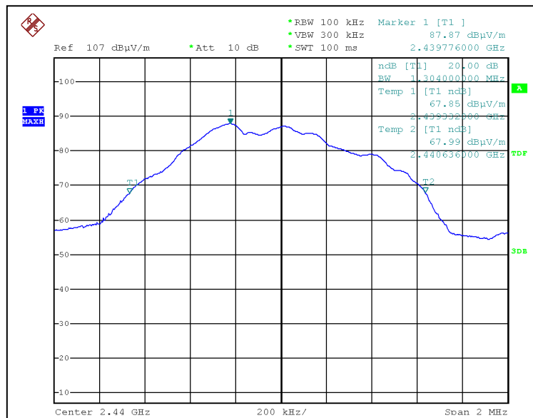
Bandwidth 2 (2440MHz)
