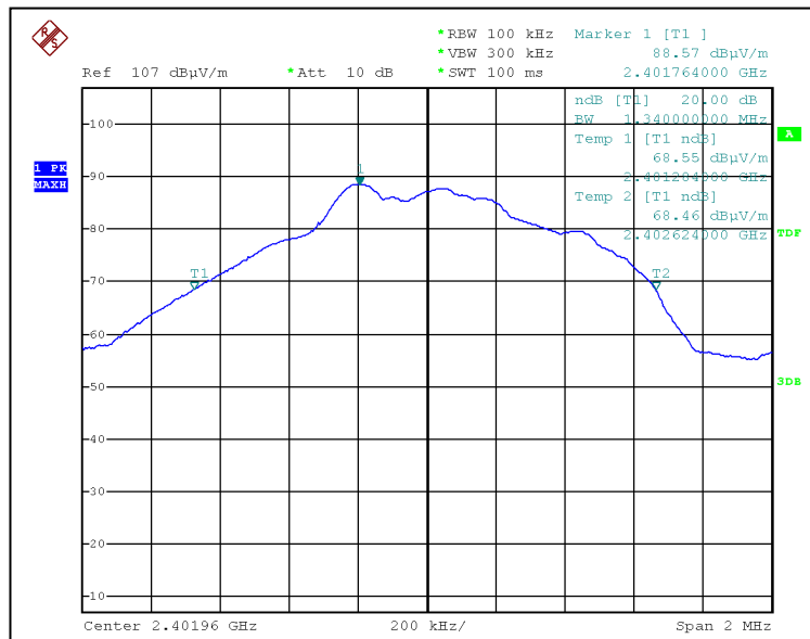
Bandwidth 1 (2402MHz)
