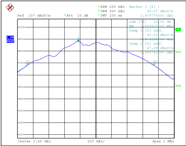
Bandwidth 3 (2480MHz)
