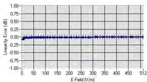
Linearity
