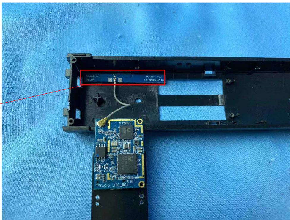
WIFI Antenna
