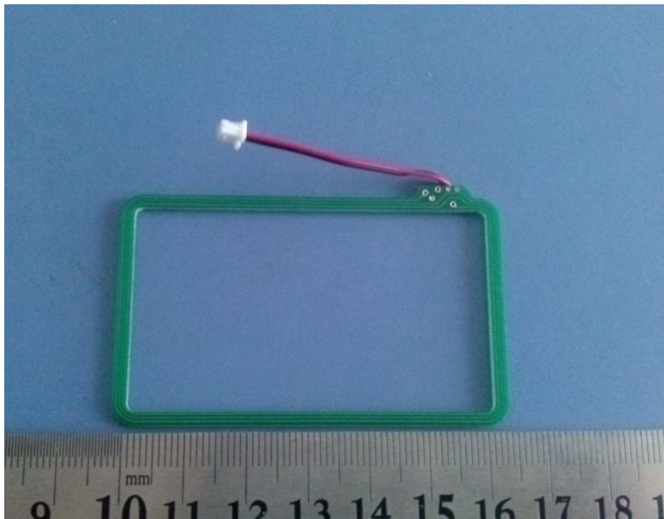
Antenna photo
