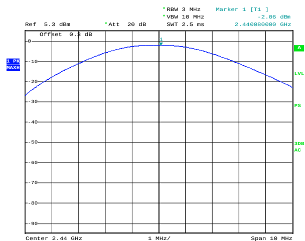
Peak Output Power (Channel 39)
