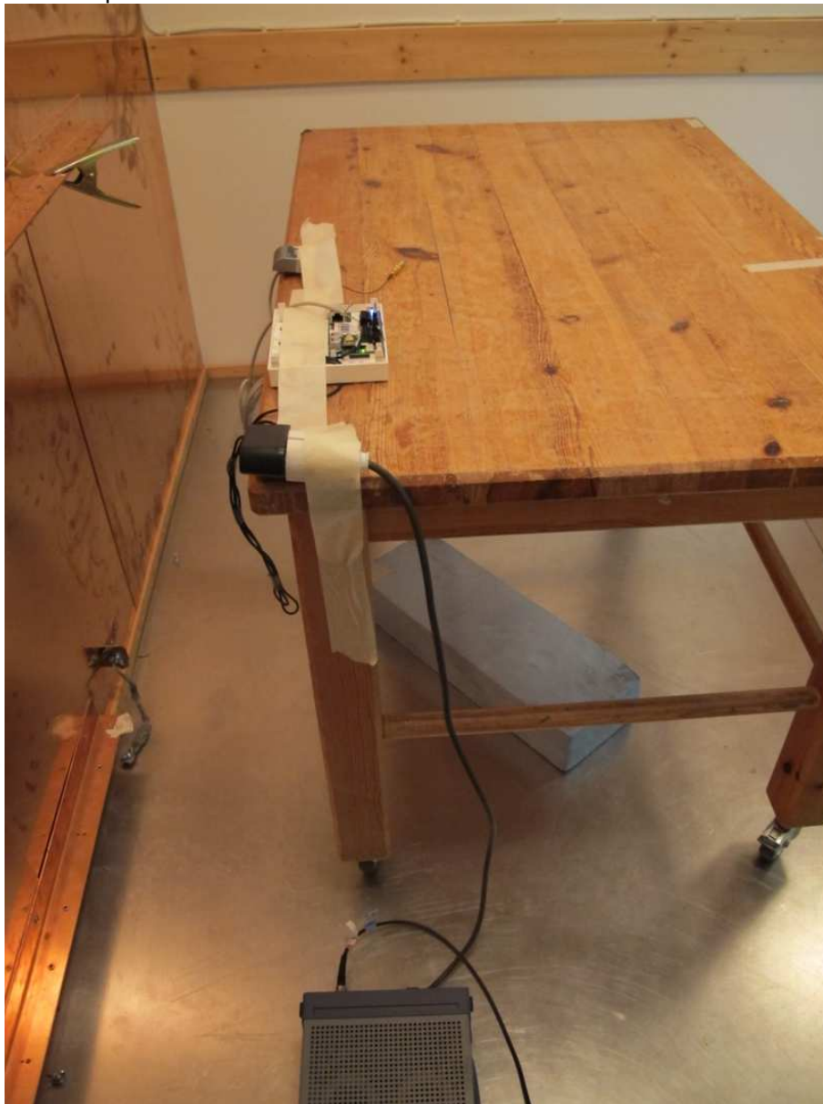
Test setup conducted emission
