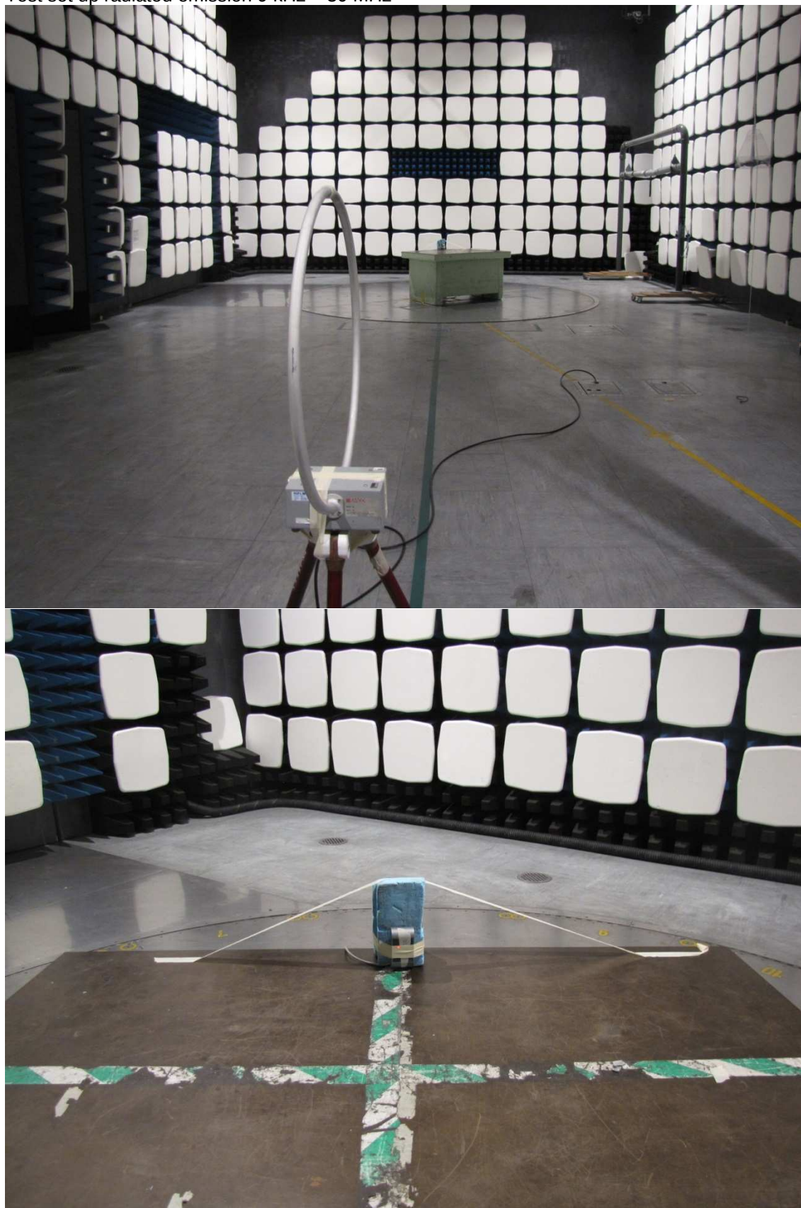
Test set up radiated emission 9 kHz – 30 MHz
