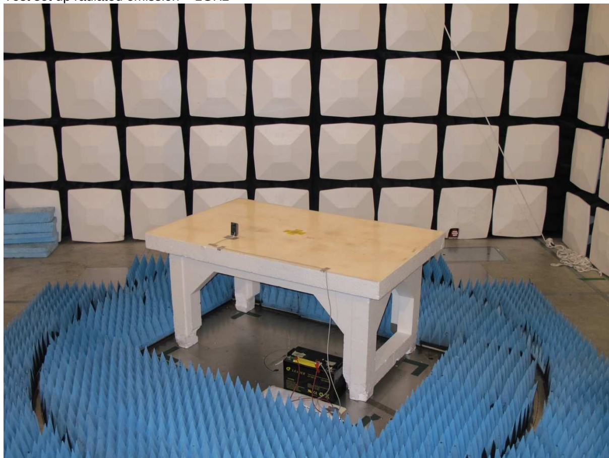
Test set up radiated emission > 1GHz
