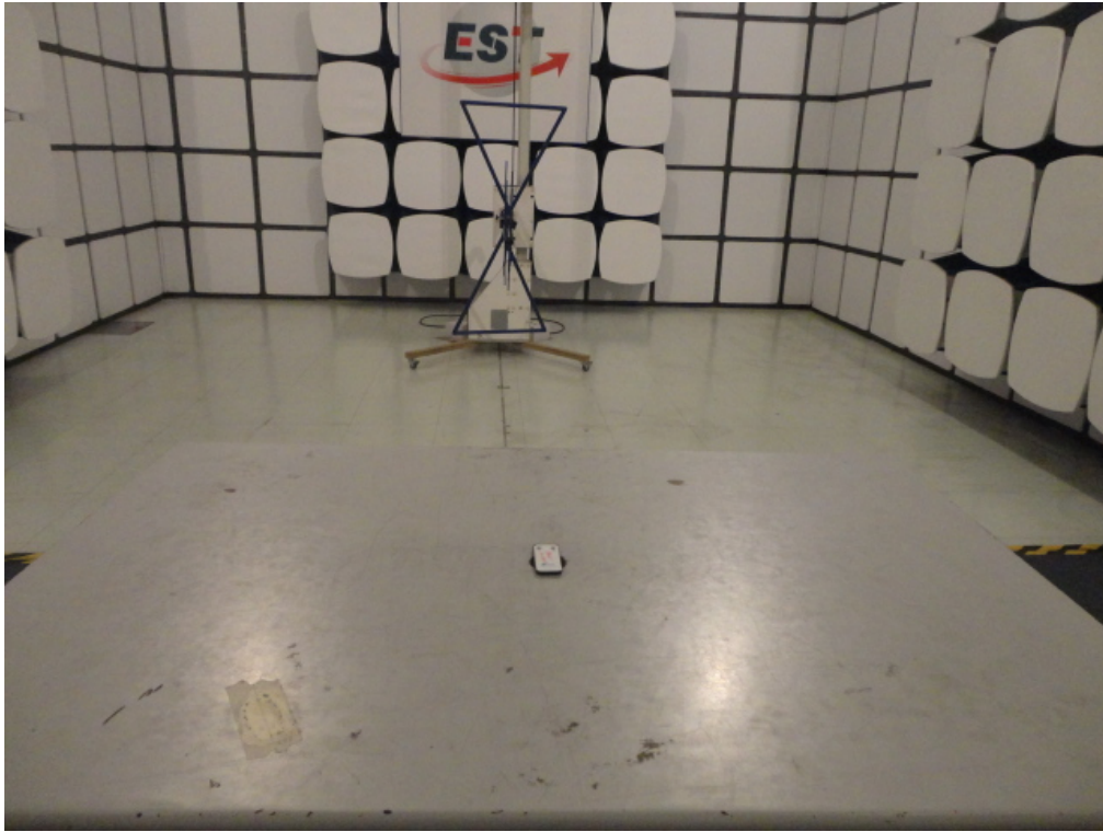
Set-up for radiated measurements (30MHz to 1000MHz)
