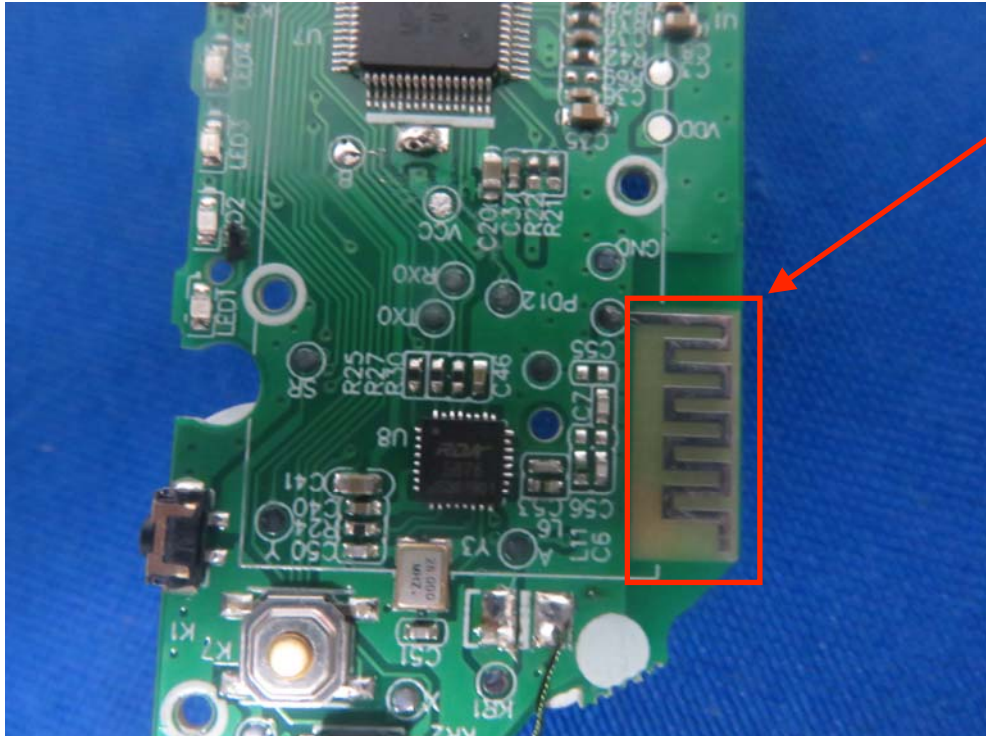
BT Antenna
