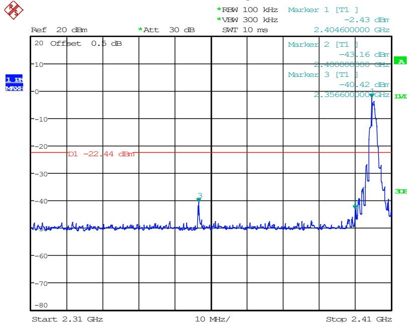
GFSK: Band Edge, Left Side
