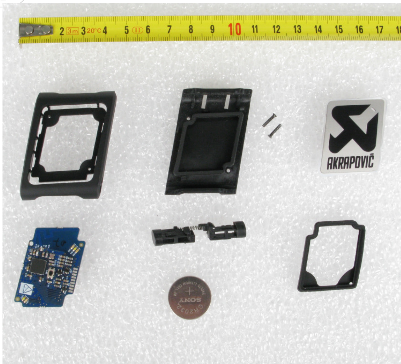
Figure 1: Top view
