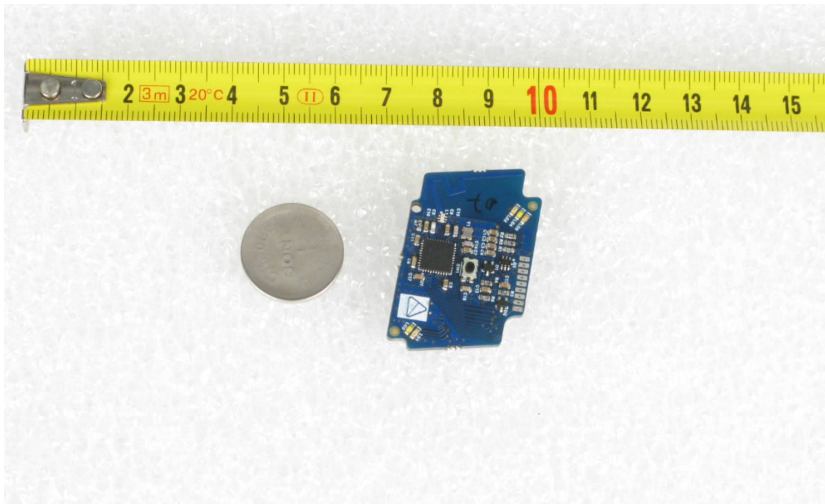
PCB board upper view
