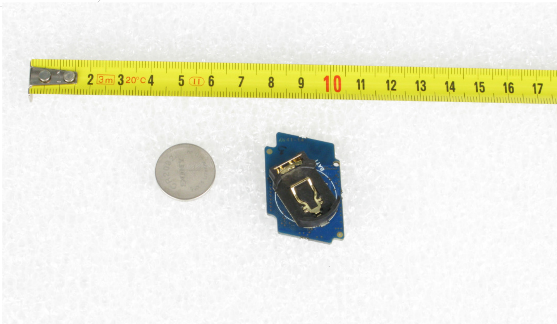
PCB board bottom view
