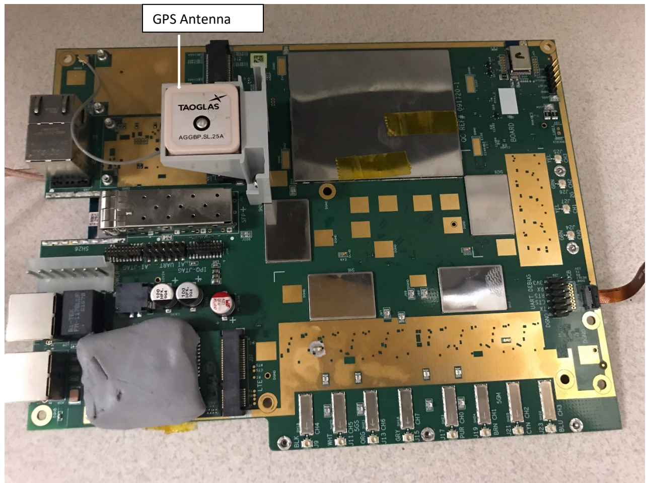
Main IPQ Board with Shields (Front)
