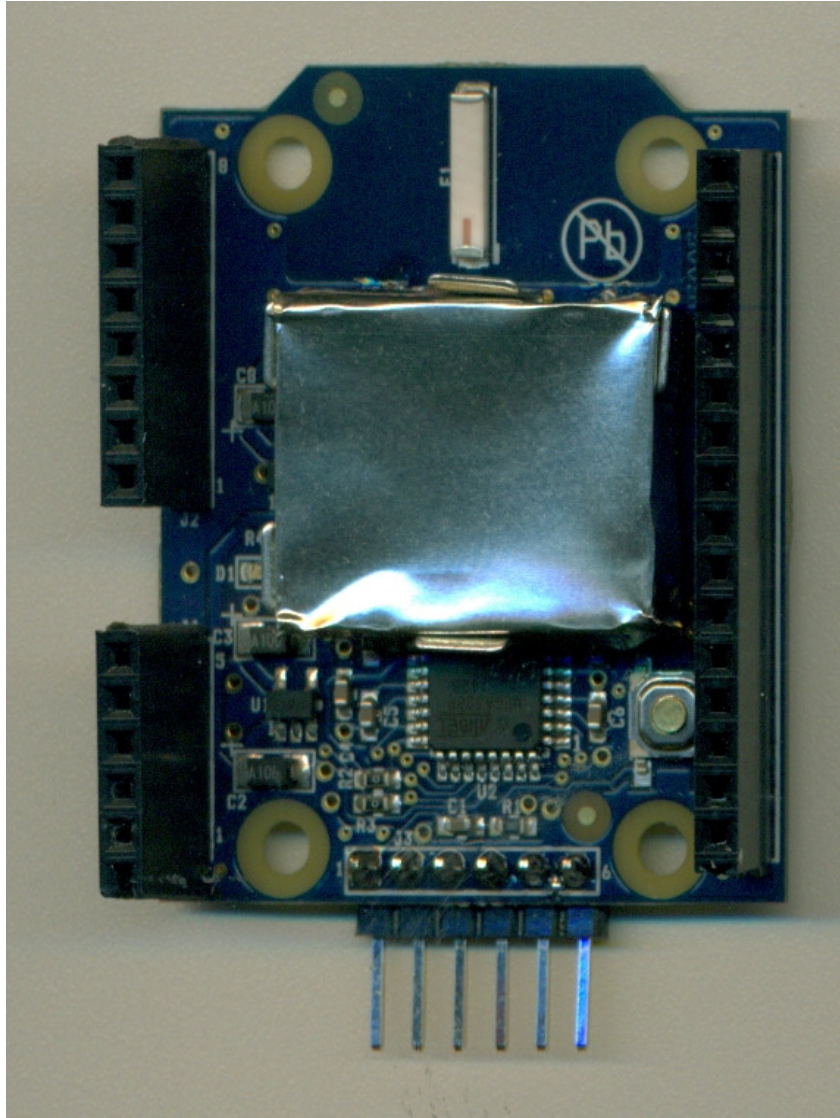
Photo 2 – Bottom View with RF Shield Cover
