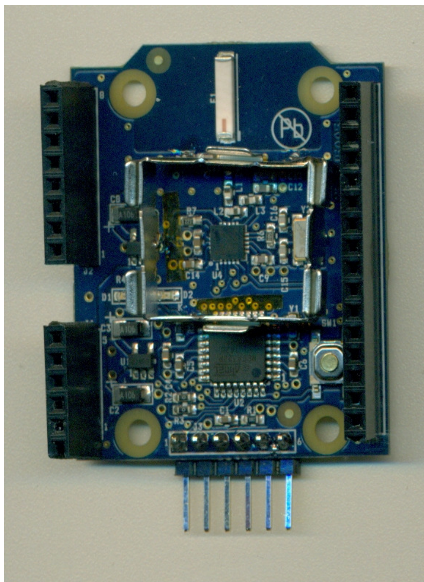
Photo 1 – Top View with RF Shield Cover Removed
