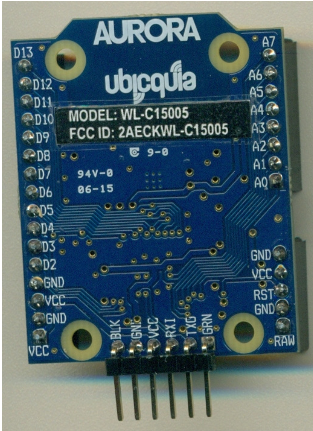
Photo 3 – Bottom View
