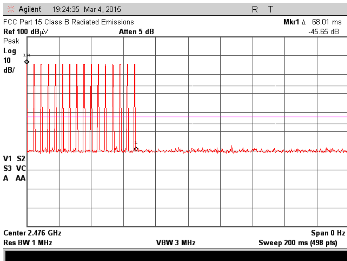
Figure 7.2-1 – Packet Duration
